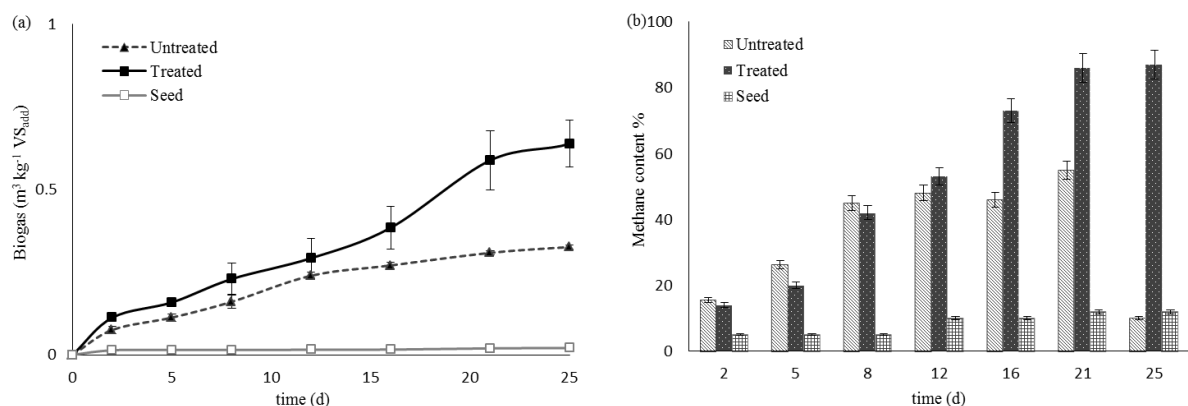
Figure 2: S. obliquus BMT cumulative biogas production (a) and percentage methane content (b) of treated and untreated algal biomass at 38°C.
