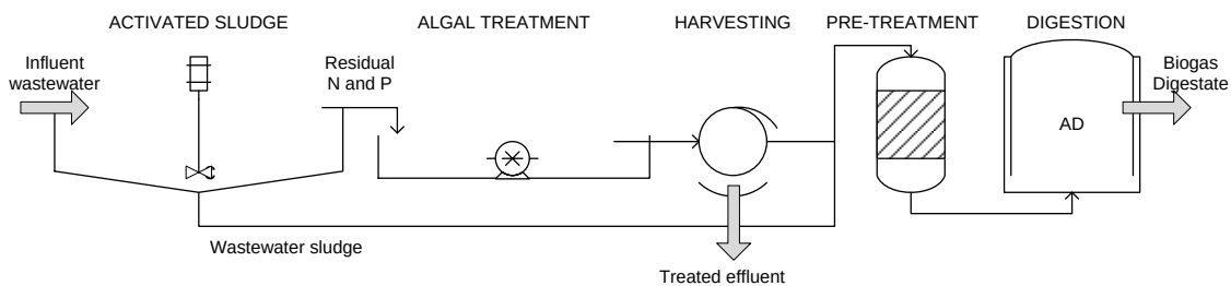
Figure 1: Schematic diagram of an integrated microalgae wastewater treatment process
