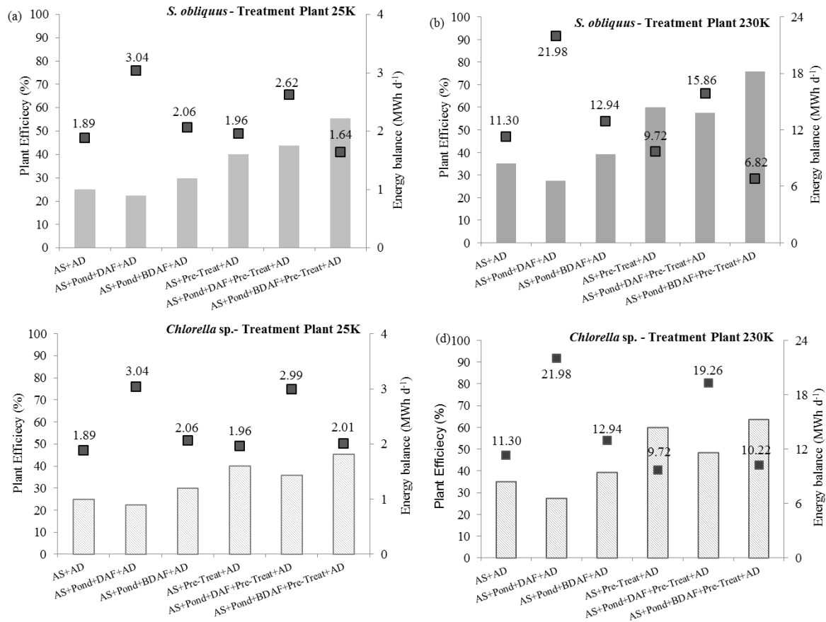
Figure 5: Plant efficiency (column) and Energy balance (square) of the scenarios: S. obliquus in TP 25K (a) and TP 230K (b); Chlorella sp. in TP 25K (c) and TP 230K (d).
