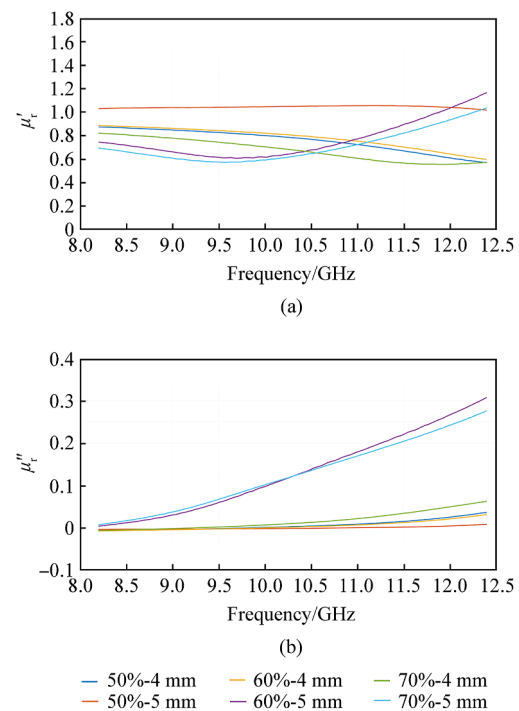
Fig. 20. Complex permeability of MnZn/epoxy samples: (a) Real part of complex permeability of MnZn/epoxy samples; (b) Imaginary part of complex permeability of MnZn/epoxy samples.
