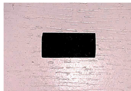
Fig. 6. Manufactured MnZn ferrite/epoxy sample.
