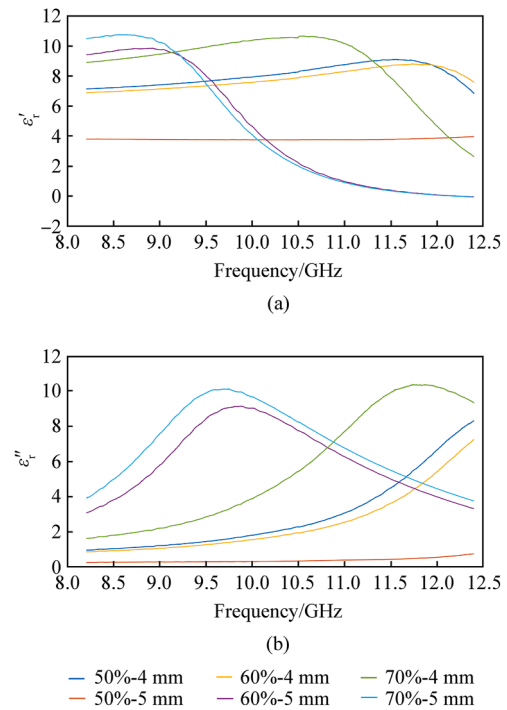
Fig. 19. Complex permittivity of MnZn/epoxy samples: (a) Real part of complex permittivity of MnZn/epoxy samples; (b) Imaginary part of complex permittivity of MnZn/epoxy samples.
