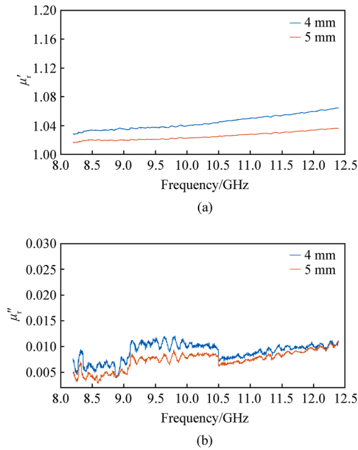
Fig. 18. Complex permeability of pure epoxy resin samples: (a) Real part of complex permeability of pure epoxy resin; (b) Imaginary part of complex permeability of pure epoxy resin.
