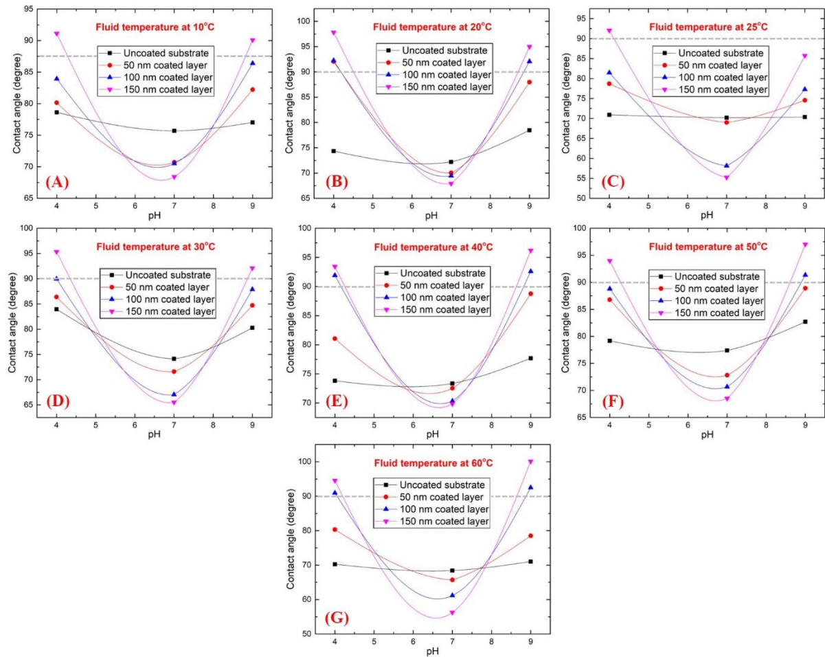
Fig. 5. Contact angle measurements of coated and uncoated Al substrates with DIW of pH 4, 7, and 9 at: (A) 10°C fluid temperature, (B) 20°C fluid temperature, (C) 25°C fluid temperature, (D) 30°C fluid temperature, (E) 40°C fluid temperature, (F) 50°C fluid temperature, and (G) 60°C fluid temperature.
