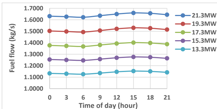
Figure 9. Time-based fuel flow at the different power setting
