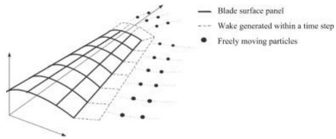
Figure 8. Typical layout of the free-wake modelling of a blade; reproduced from Ref. [53]
