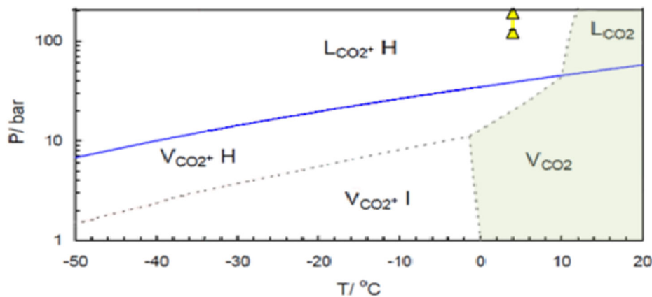
Fig. 18. Hydrate formation in pure saturated carbon dioxide system [151]; 'L' indicates a liquid-rich zone; 'V' indicates a vapour-rich zone; 'T' indicates an area where dry-ice will form; 'H' indicates the hydrate-stability zone; the yellow triangles represent CO 2 pipeline condition. (For interpretation of the references to colour in this figure legend, the reader is referred to the web version of this article.)
