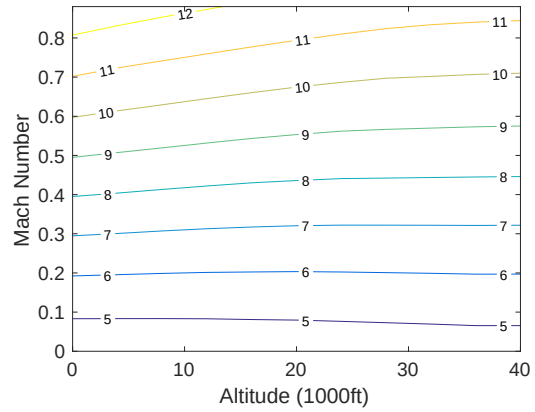
(b) Specific fuel consumption (mg/Ns)
