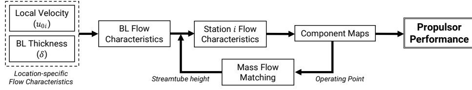
Figure 4: BLI propulsor simulation method at off-design
