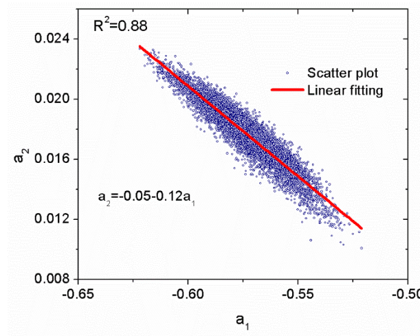
Fig. 6: The plot of the second order coefficient a_2 as a function of the first order coefficient a_1 for one damage-free specimen.
