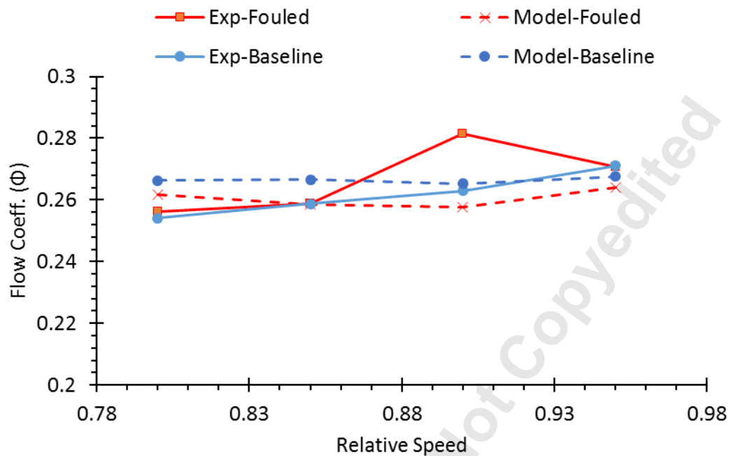
Fig. 11 Disturbance mean flow coefficient for baseline and fouled operations
