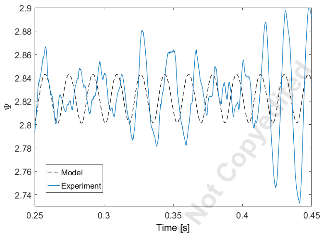
Fig. 13 Measured time waveform for the plenum pressure-rise coefficient at 0.85 of rated speed
