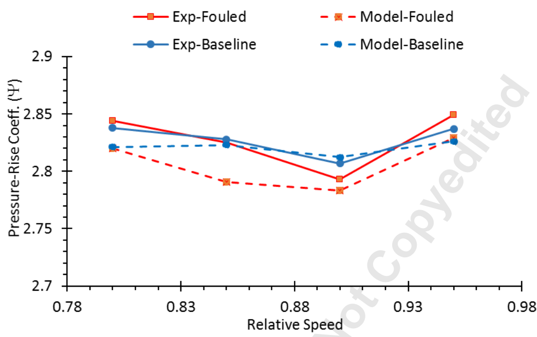
Fig. 12 Disturbance mean pressure-rise coefficient for baseline and fouled operations
