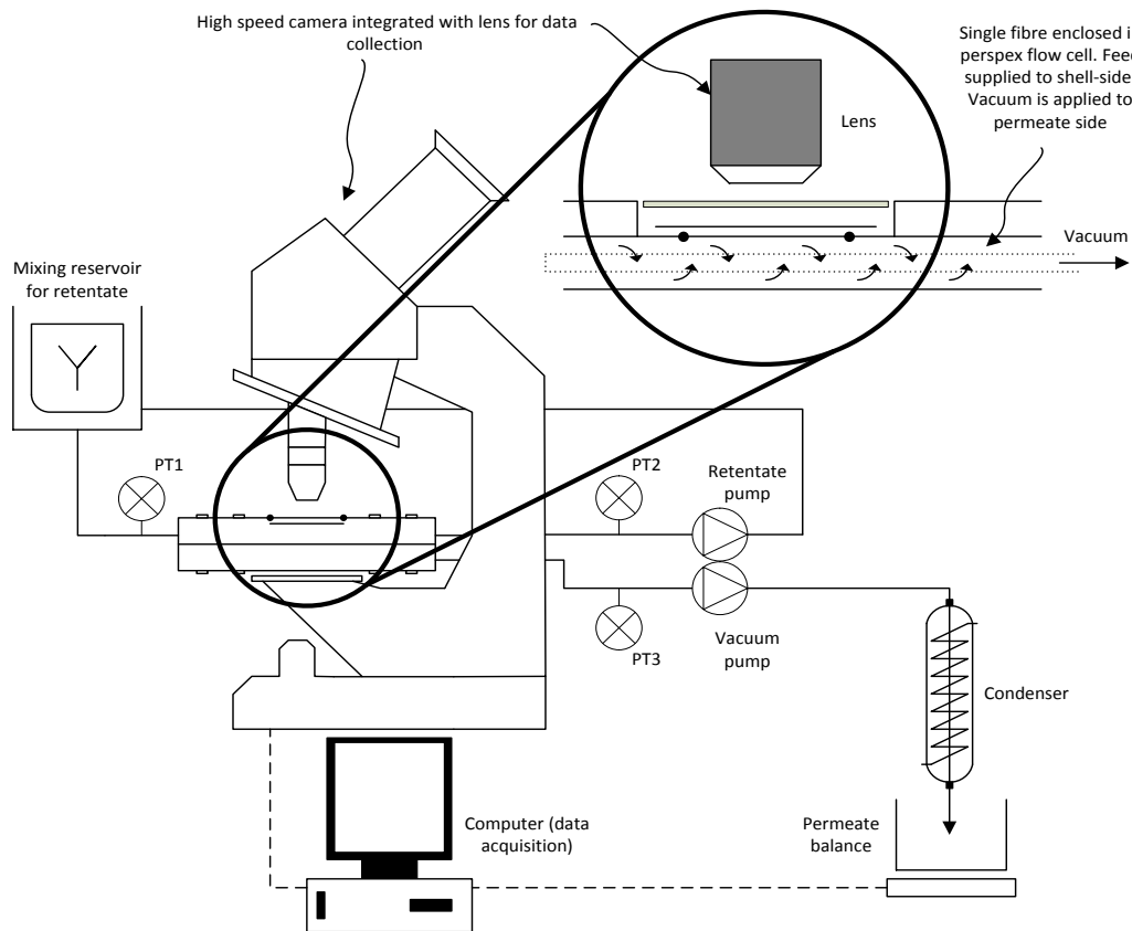
Figure 1. Experimental set-up.
