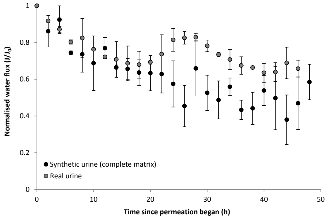
Figure 3. Flux variation during the vacuum membrane distillation of real urine. Feed temperature= 60 °C, Cross flow velocity = 0.11 \text{ m s}^{-1} , Initial flux J_0 = 3.05 \text{ L m}^{-2} \text{ h}^{-1} , vacuum degree= 40 mBarA.
