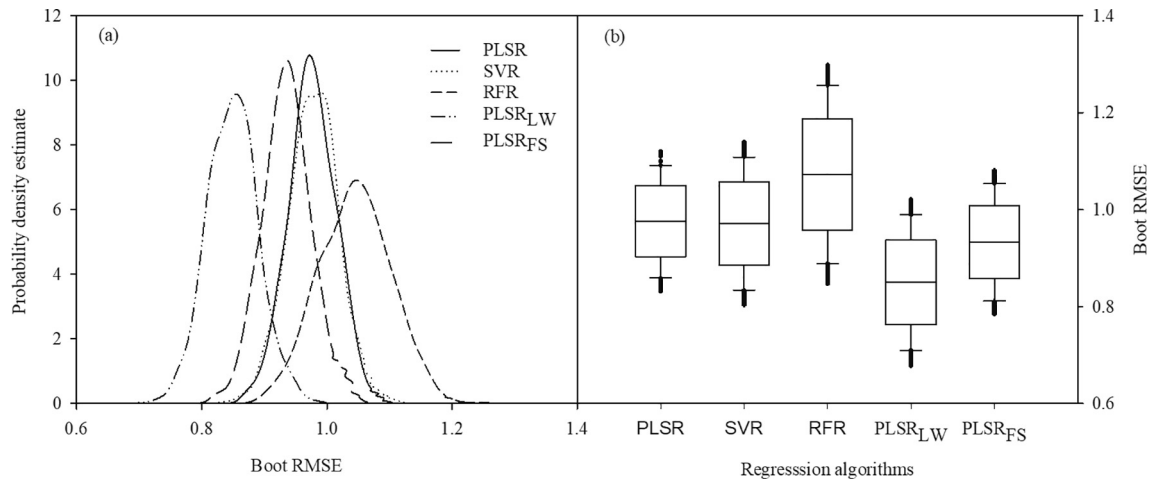
Fig. 4 – Distribution of (a) probability density function (pdf) estimated by kernel density estimator of the 1000 RMSE values and (b) the boxplots with median, lower quartile and upper quartile from all the boot strapped calibration approaches used for estimating LAI.
