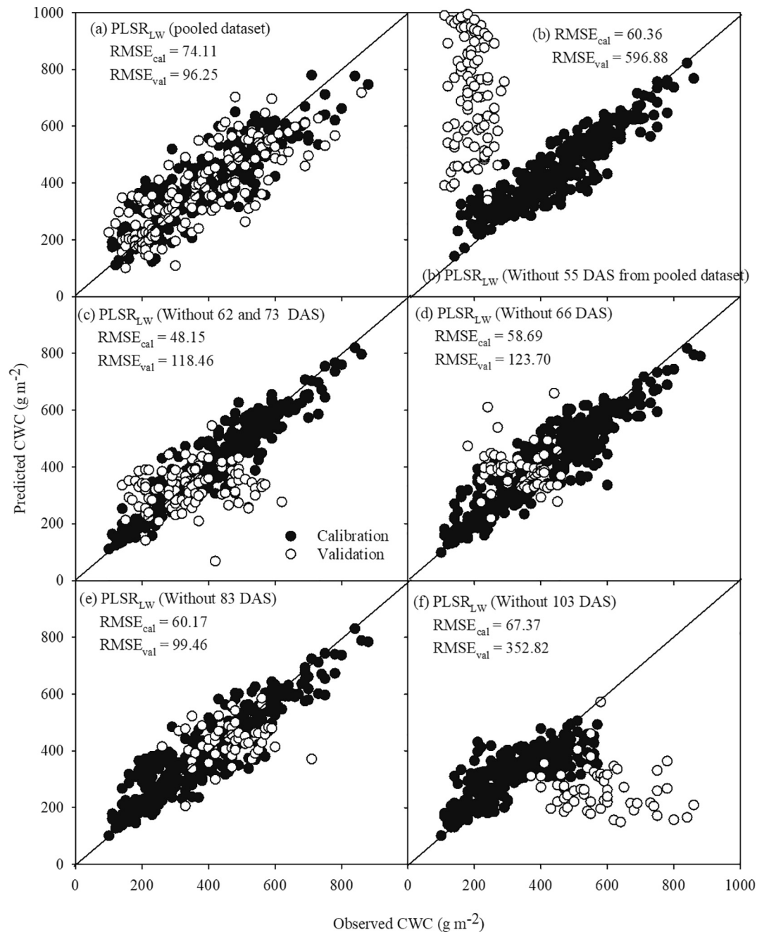
Fig. 8 – Scatter plot between calibration and validation datasets of CWC ( \text{g m}^{-2} ) for \text{PLSR}_{\text{LW}} model with removal of a specific date (DAS) from each year dataset.
