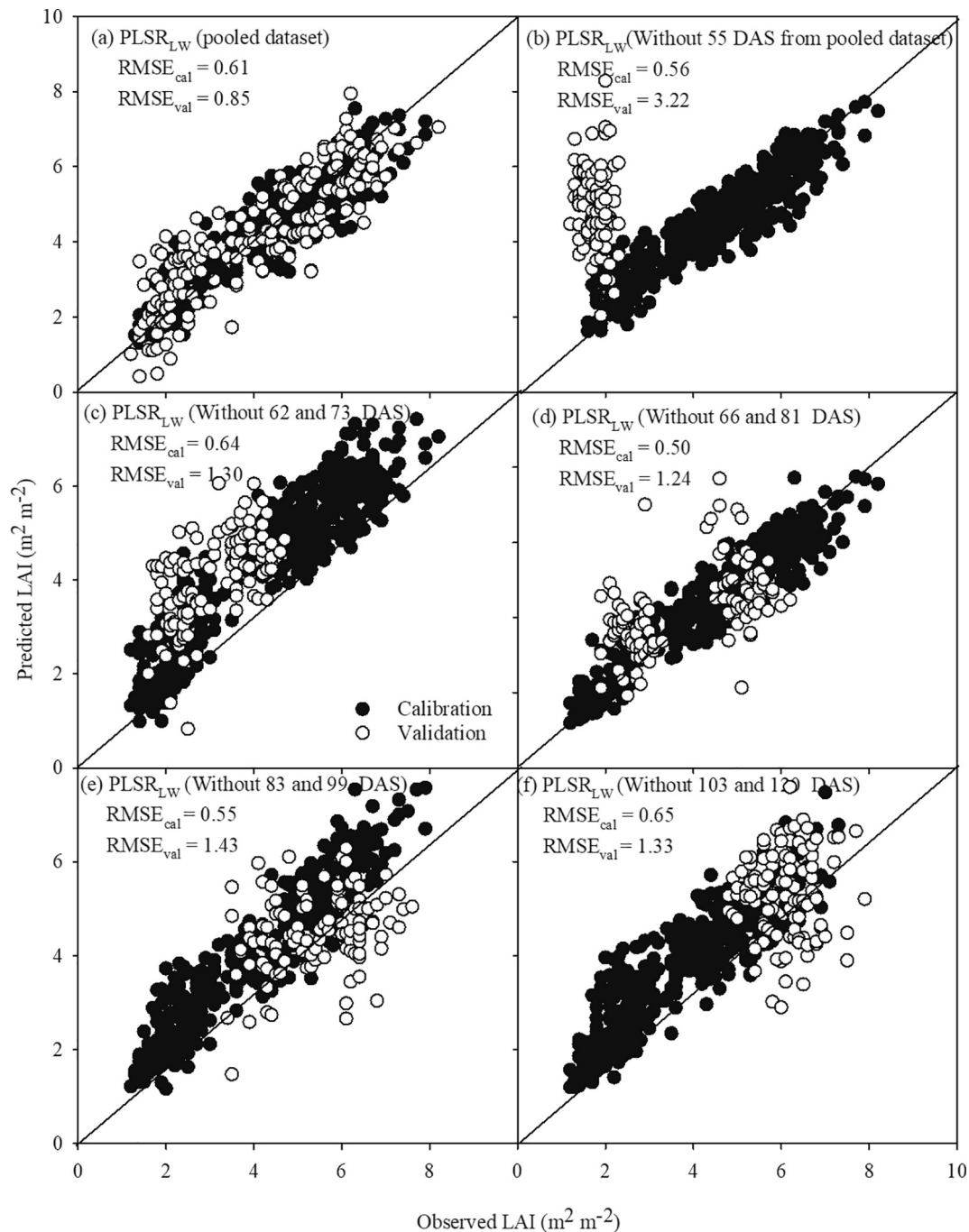
Fig. 7 – Scatter plot between calibration and validation datasets of LAI ( \text{m}^2 \text{m}^{-2} ) for \text{PLSR}_{\text{LW}} model with removal of a specific date (DAS) from each year dataset.
