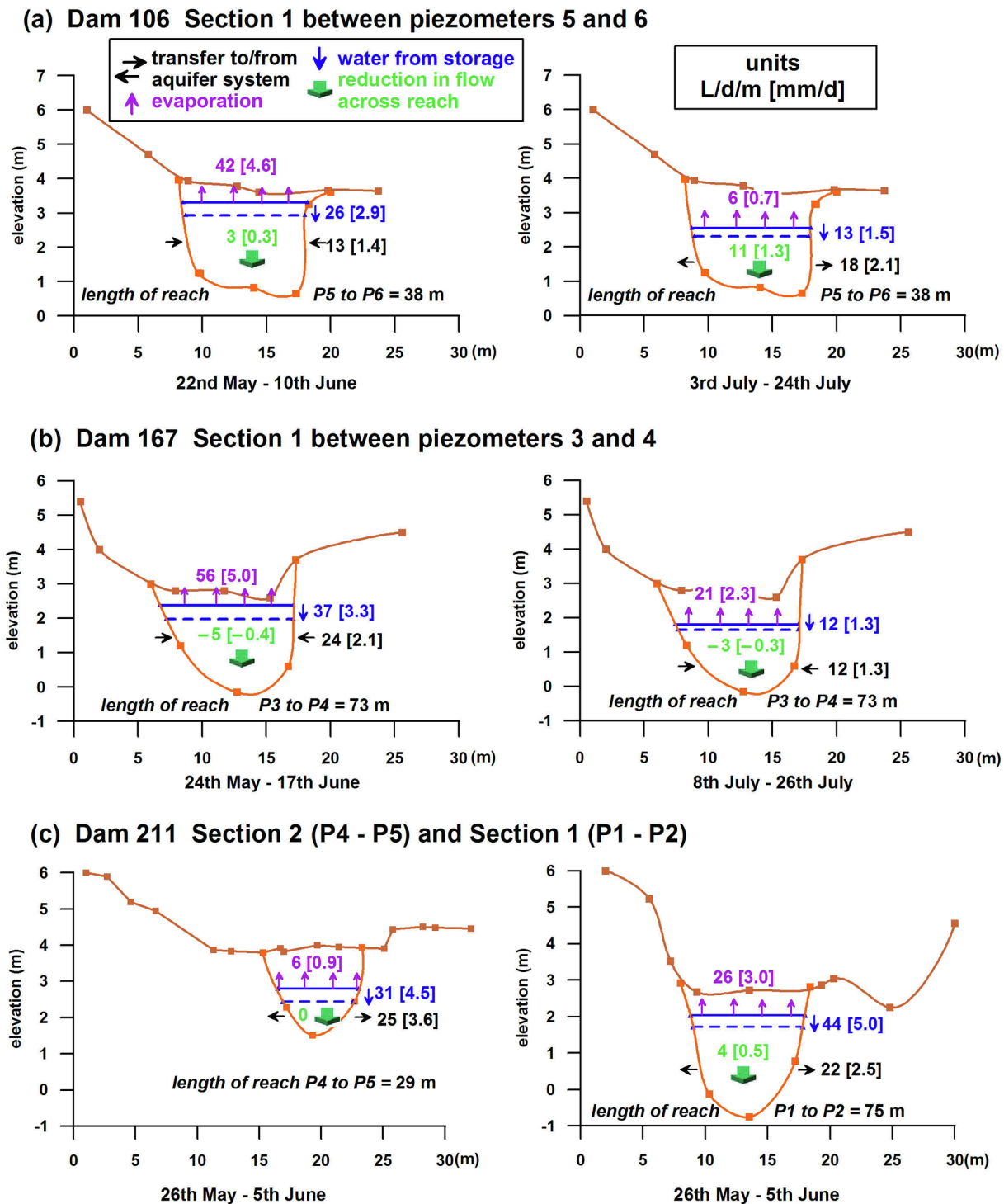
Fig. 8. Selected water balances for certain reaches (a) Dam 106 Section 1 between piezometer 5 and 6 (b) Sam 167 Section 1 between piezometer 3 and 4 (c) Dam 211 section 2 (P4–P5) and Section 1 (P1–P2); units L/d/m and [mm/d].
