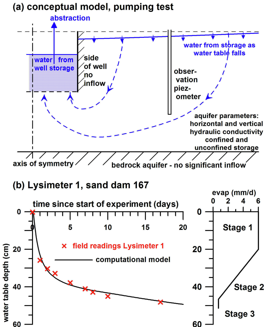
Fig. 3. Estimation of aquifer parameters and rate of evaporation from sand: (a) conceptual model for pumping from a partially penetrating well open at its base, (b) representation using a semi-empirical model of a lysimeter experiment.
