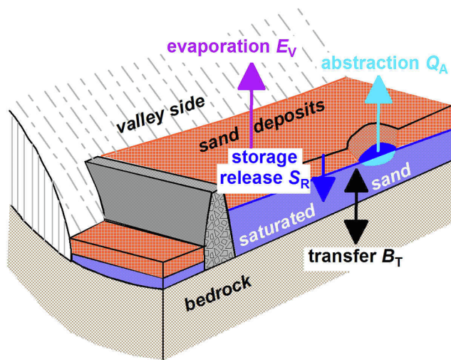
Fig. 1. Schematic diagram of a sand dam showing important flow components during the dry season.
