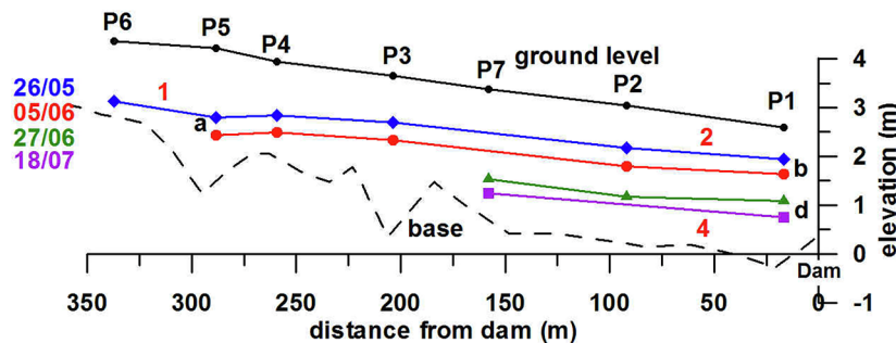
Fig. 4. Water table elevations in the deposited sand for each study area (P = piezometer). (a) Sand dam 106, (b) sand dam 167 and (c) sand dam 211. Letters a to d signify where the rate of fall in the water level is recorded; numbers 1–4 in red indicated where the slope in the water table is calculated. (For interpretation of the references to colour in this figure legend, the reader is referred to the web version of this article.)
