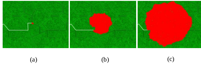
Figure 6: Illustration of (a) 1st (b) 25th (c) 50th contours around the crack tip for a deviating crack
