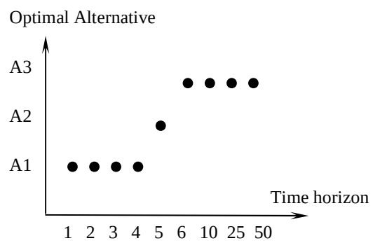
Figure 7 Optimal Alternatives.
