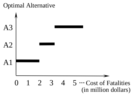
Figure 6 Optimal retrofit alternative as one varies N_L V , given discount rate 5%.
