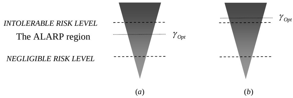
Figure 3 (a) C_{Opt} is acceptable only if \gamma_{Opt} is smaller than the unacceptable risk level (most possibly within the ALARP region) (b) If \gamma_{Opt} is within the unacceptable risk region, an alternative with expenditure C ( C > C_{Opt} ) which will lead to an acceptable value of risk is preferred.
