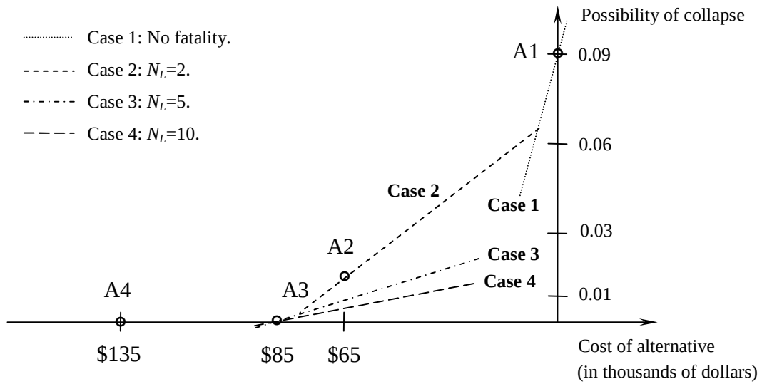
Figure 4 Computation of the optimal alternative. Alternative A1 is optimal in case 1; A2 is optimal in case 2; A3 is optimal in case 3 and 4.
