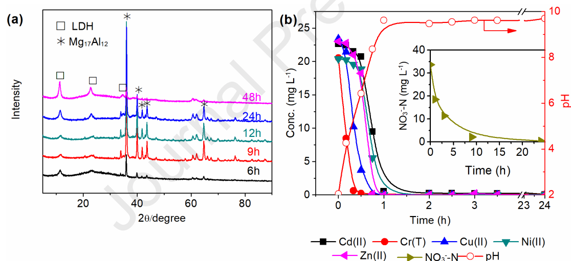
Fig. 7. Effect of reaction time on hydrolysis products and heavy metals and nitrate concentration for Mg-Al alloy and contaminated water. (a) XRD characterization of reaction products, (b) heavy metals and NO_3^- concentration and pH variation. Mg-Al alloy 3 g, contaminated water 300 mL, initial pH = 2, stirring speed 300 rpm, temperature 22 \pm 2 °C.
