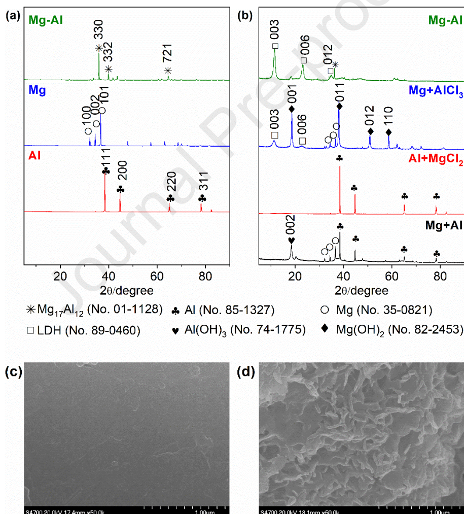
Fig. 2. (a, b) XRD and (c, d) SEM characterization. (a) Mg and Al metals and Mg-Al alloy, (b) the hydrolysis products of Mg-Al alloy, Mg+AlCl 3 , Al+MgCl 2 and Mg+Al at initial pH 2 (HCl), (c) Mg-Al alloy, (d) the hydrolysis product of Mg-Al alloy. 3 g Mg-Al alloy (Mg/Al = 60/40), particle size >200 meshes; 3 g Mg metal powders (>240 meshes) in AlCl 3 solution (100 mg L -1 Al 3+ ), 3 g Al metal powders (>325 meshes) in MgCl 2 solution (200 mg L -1 Mg 2+ ), 1.8 g Mg metal powders and 1.2 g Al metal powders. Aqueous solution volume 300 mL, made to pH 2 (HCl), hydrolysis time 24 h, stirring speed of magnetic bar 300 rpm, temperature 22 °C±2 °C.
