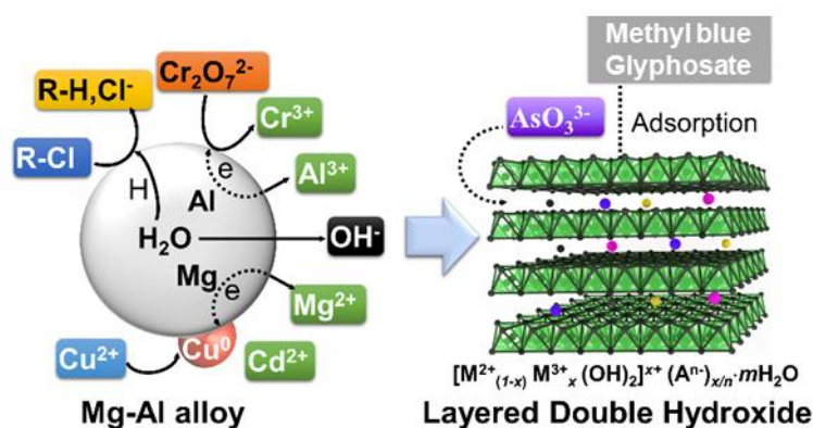
Fig. 1 Schematic illustration of model pollutants removal by Mg-Al alloy in situ layered double hydroxide from contaminated water.
