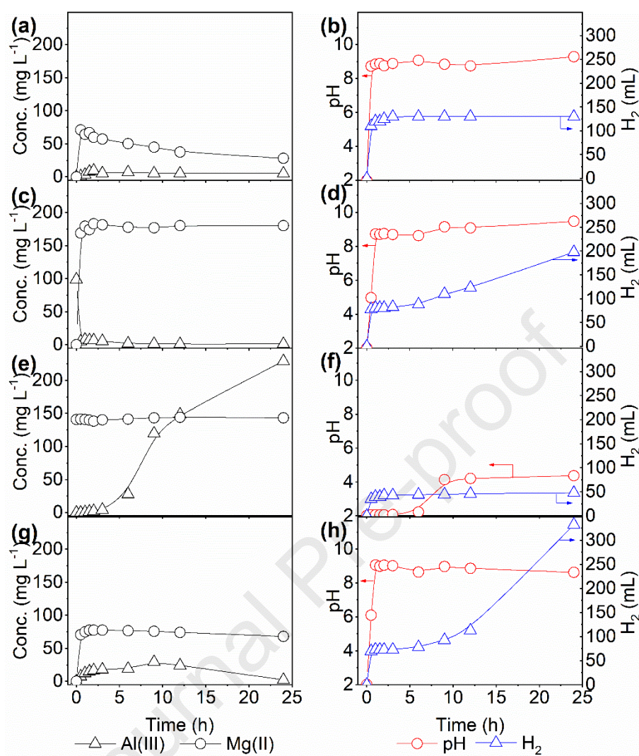
Fig. 3. Mg and Al ion concentration, pH and hydrogen generation in the experiment of Fig. 2. (a, b) Mg-Al alloy, (c, d) \text{Mg} + \text{AlCl}_3 , (e, f) \text{Al} + \text{MgCl}_2 and (g, h) \text{Mg} + \text{Al}
