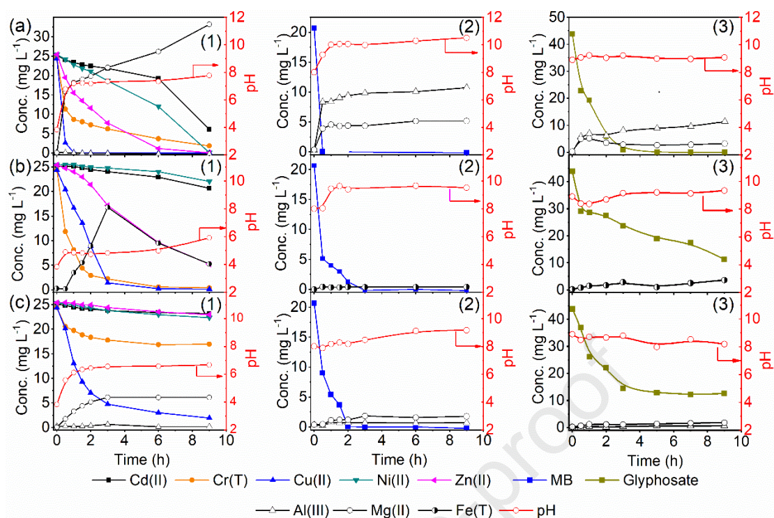
Fig. 9. Concentrations of pollutants (heavy metals, methyl blue and glyphosate), leached concentrations of Mg, Al and Fe ions, and pH variations at initial pH 3.5 (left panel), pH 8.0 (middle) and 9.0 (right). (a) Mg-Al alloy, (b) ZVI, (c) LDH. Materials 3 g, contaminated water 300 mL, reaction time 9 h, stirring speed 300 rpm, temperature 22 °C±2 °C.
