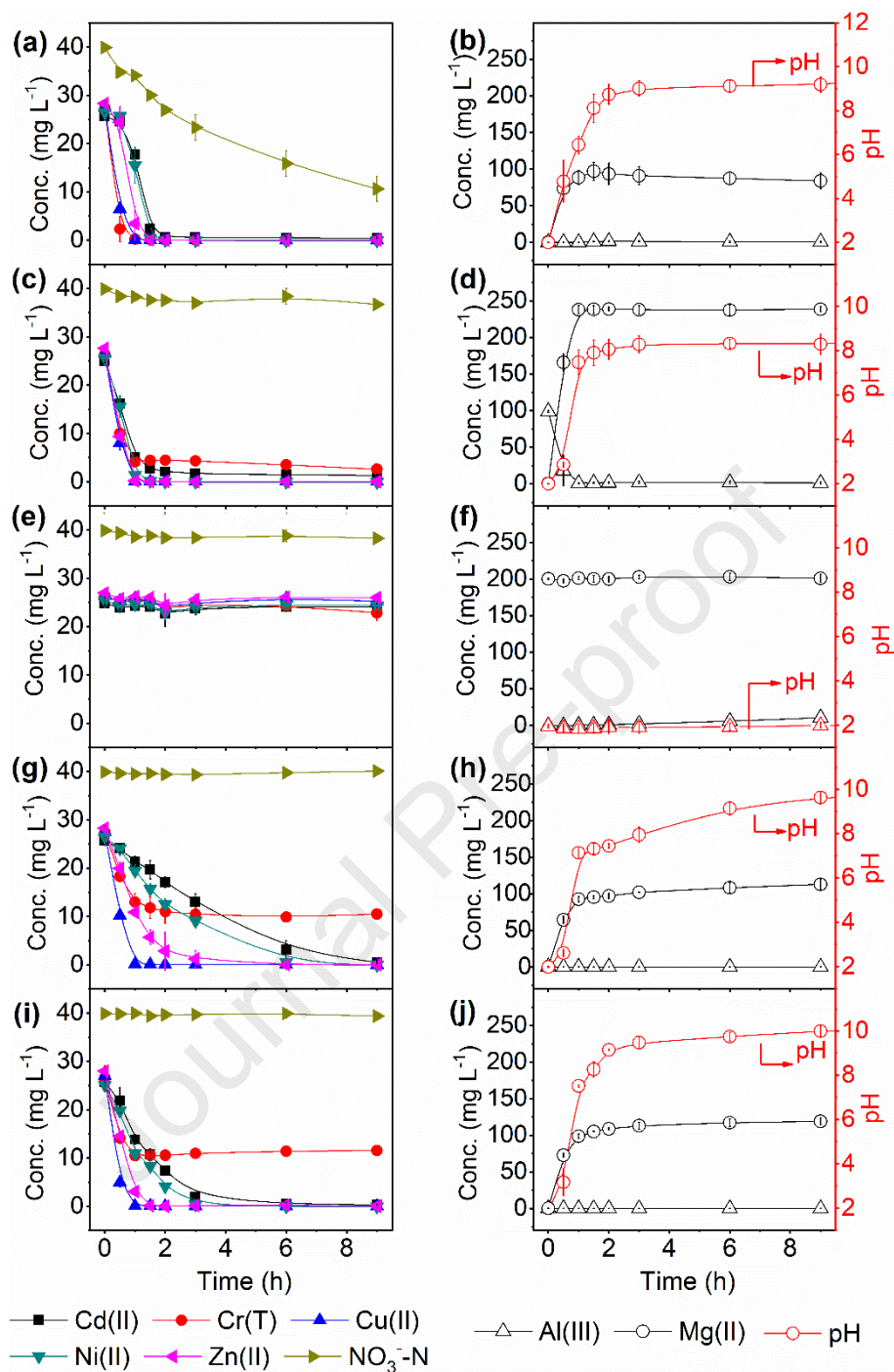
Fig. 4. Concentrations of heavy metals, nitrate, Mg and Al ions and the pH of solution as a function of reaction time in contaminated water (300 mL, pH 2). (a, b) Mg-Al alloy, (c, d) Mg+AlCl 3 , (e, f) Al+MgCl 2 , (g, h) Mg+Al, (i, j) Mg. Stirring speed 300 rpm, temperature 22 °C±2 °C, concentration of individual heavy metal 25 mg L -1 , nitrate 40 mg L -1 , other experimental condition is the same as Fig. 2. The results are the average of three independent experiments with the standard deviation as the error bar.
