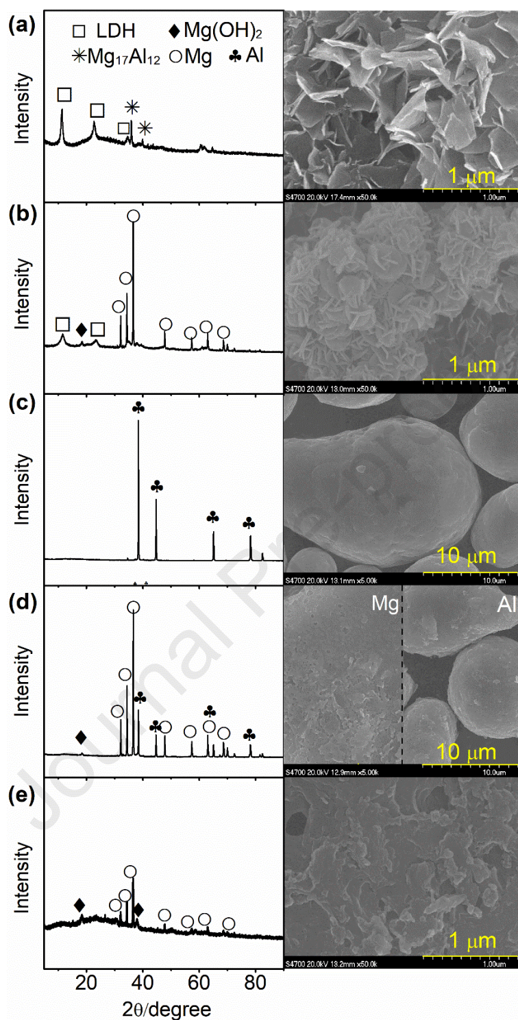
Fig. 5. XRD and SEM characterization of the materials after reaction with contaminated water as in Fig. 4. (a) Mg-Al alloy, (b) Mg+ \text{AlCl}_3 , (c) Al+ \text{MgCl}_2 , (d) Mg+Al, (e) Mg.
