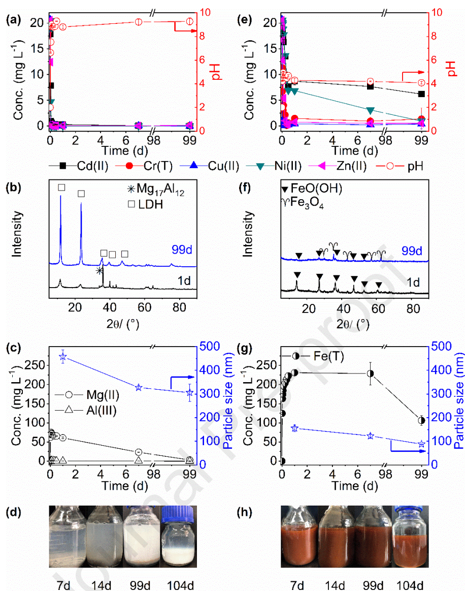
Fig. 8. Effect of reaction time on heavy metals, Al, Mg and Fe concentrations, pH and the particle size and settlement of the hydrolysis products. (a-d) Mg-Al alloy, (e-h) ZVI. Mg-Al alloy (>200 meshes, 3 g), ZVI (100-120 meshes, 3 g), contaminated water 300 mL pH 2 (HCl). The system was stirred at 300 rpm for 12 h and then stood without stirring for 99 days. Then, the suspensions were decanted to a new bottle and stood for additional 15 days. Temperature was 22 °C±2 °C.
