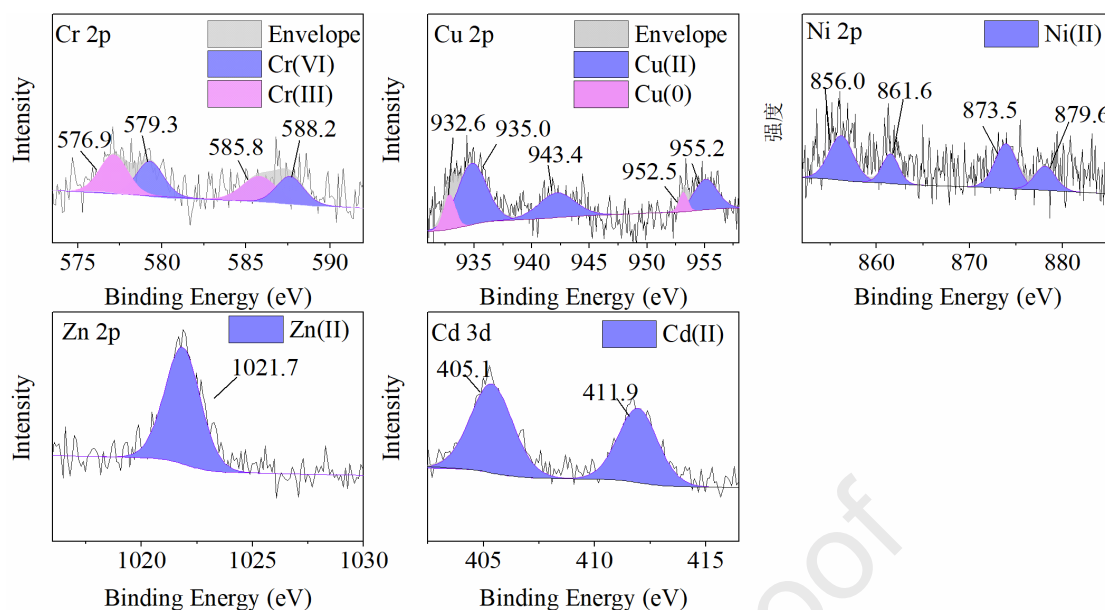
Fig. 6 XPS characterization of the reaction products of Mg-Al alloy with contaminated water. Contaminated water 300 mL, Mg-Al alloy 3 g, stirring speed 300 rpm, temperature 22 \pm 2 °C.
