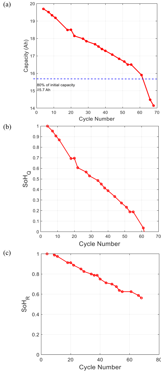
Fig. 6. (a) EoL definition based on 20% capacity fade. (b) \text{SoH}_Q : SoH of the 19-Ah Li-S cell calculated based on capacity fade. (c) \text{SoH}_R : SoH of the 19-Ah Li-S cell calculated based on power fade.
