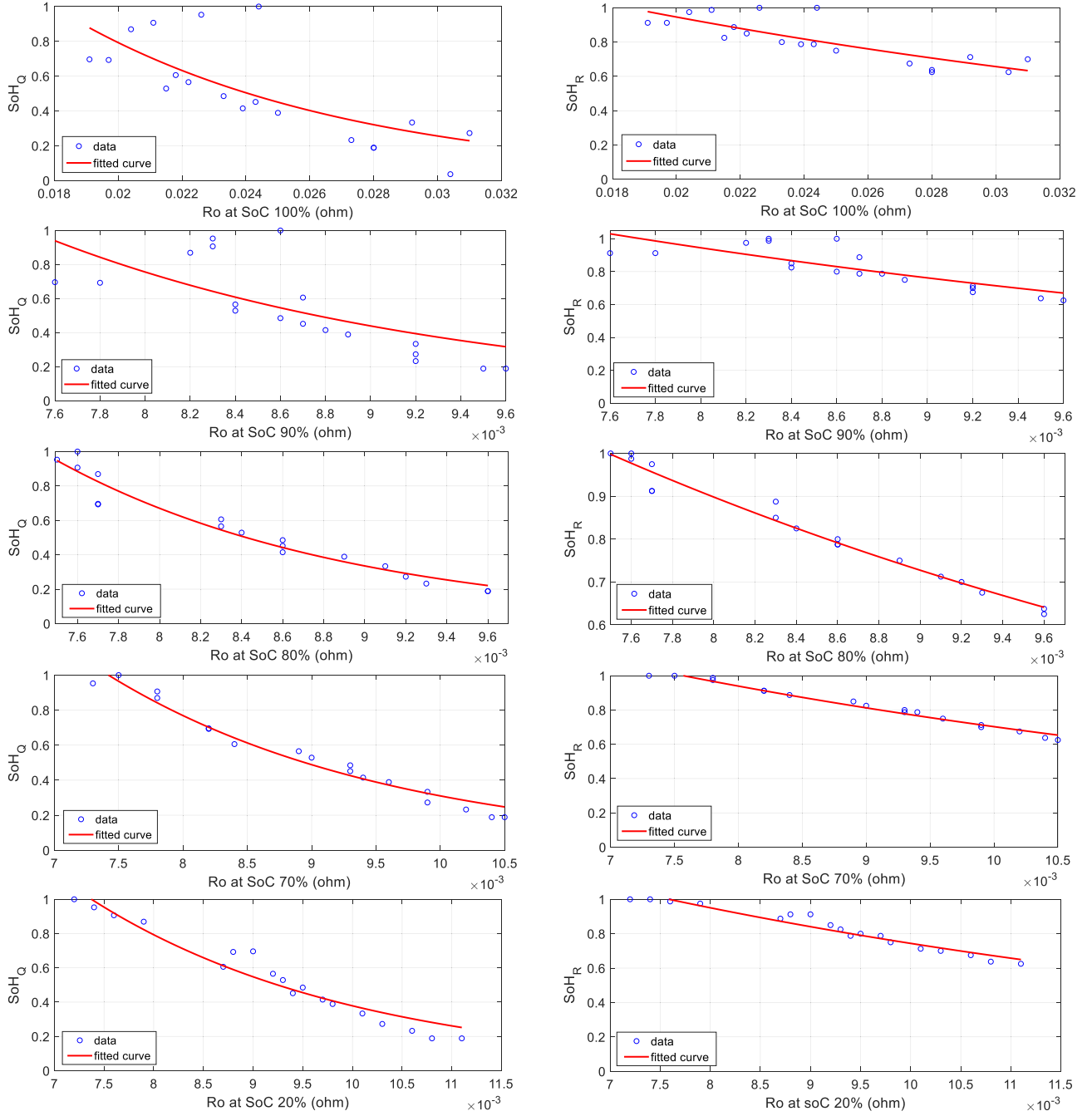
Fig. 8. Curve fitting for SoH_Q and SoH_R estimators design using training data— R_o at different SoC levels.
