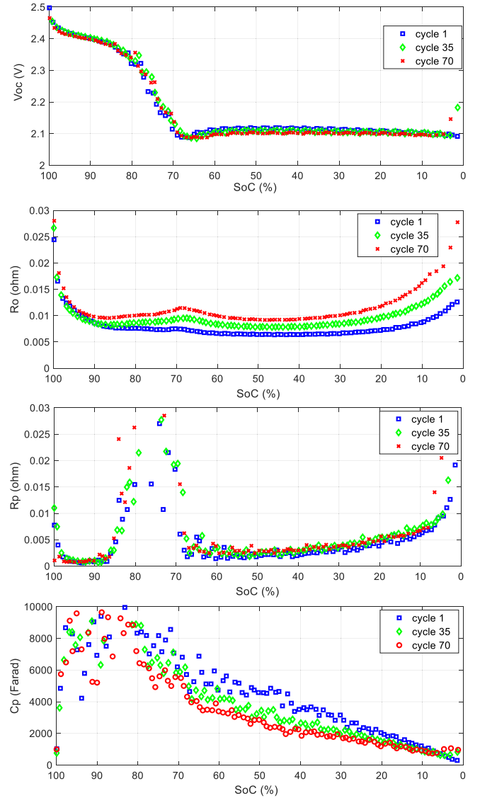
Fig. 2. Li-S cell Thevenin model's parameters versus SoC at different age levels.
