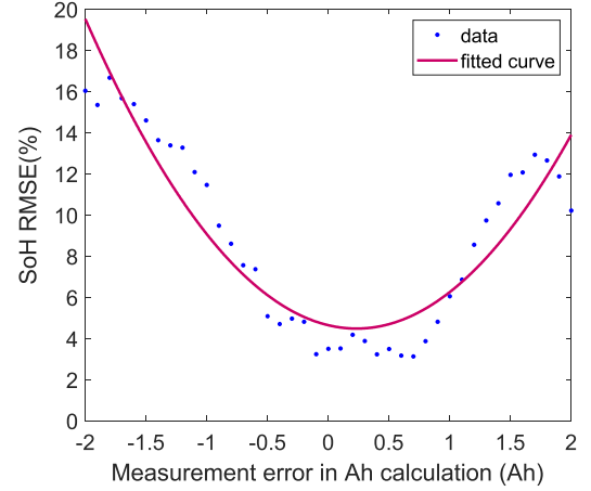
Fig. 11. Sensitivity of SoH Q estimation RMSE to UAH measurement error.
