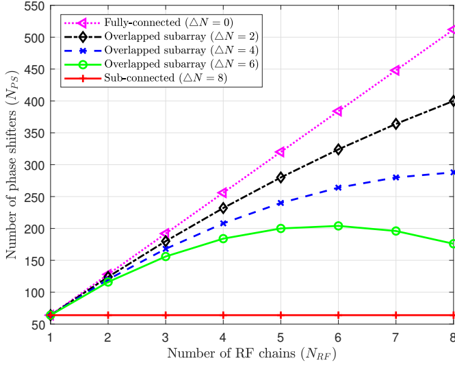
Figure 3. Number of PSs required for different structures ( N_{TX} = 64 )
