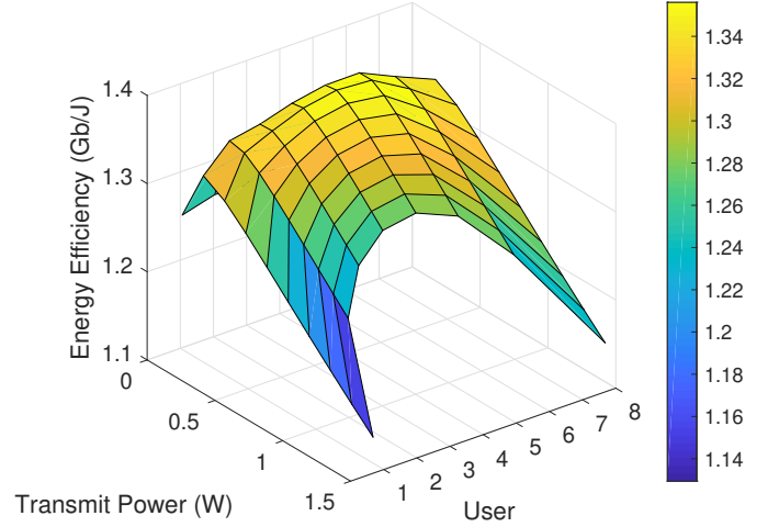
Figure 9. Energy efficiency vs transmit power for each user ( \Delta N = 4 )
