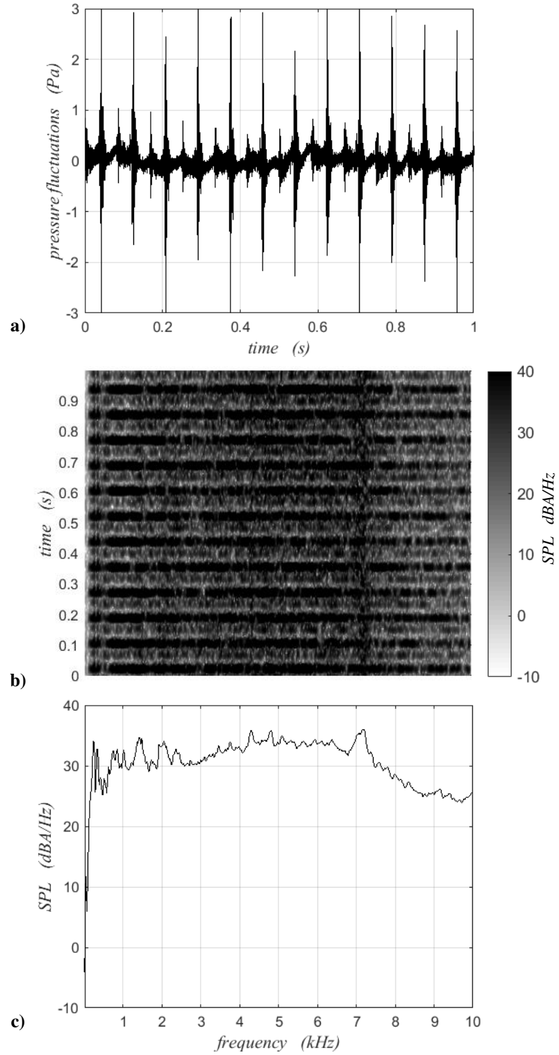
Fig. 6 Sound measured at 0° of the A wings flapping at 12 Hz: a) timetrace of the pressure fluctuations; b) A-weighted SPL spectrogram; c) A-weighted SPL spectrum.
