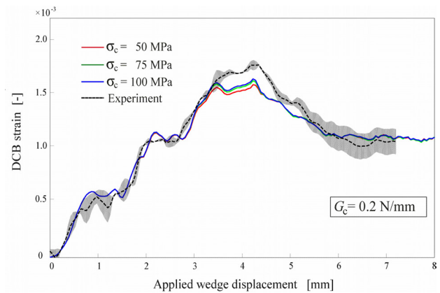
Fig. 3. Effect of strength on strain-displacement response.
