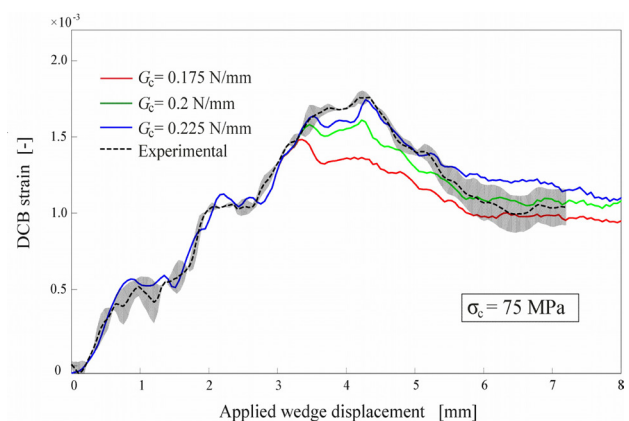
Fig. 4. Effect of fracture energy on strain-displacement response.
