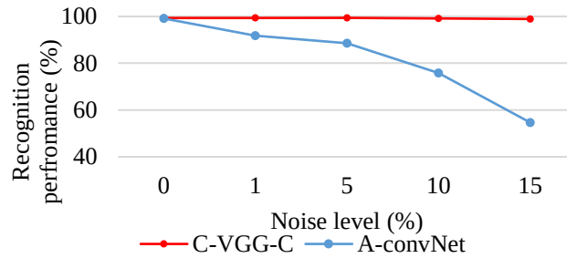
Fig. 8 Robustness in various noise levels
