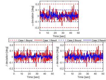
Fig. 6. CRMPC results: State deviation profiles for cases 1 and 2.
