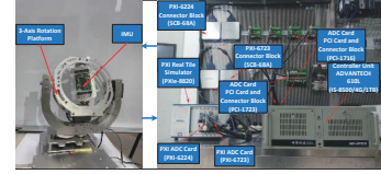
Fig. 1. Experimental platform.
