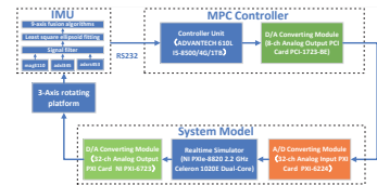
Fig. 1. Experimental platform.
