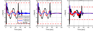
Fig. 4. Angular-rate-evolution profiles obtained via DLMPC [2], CRMPC, and LQR.
