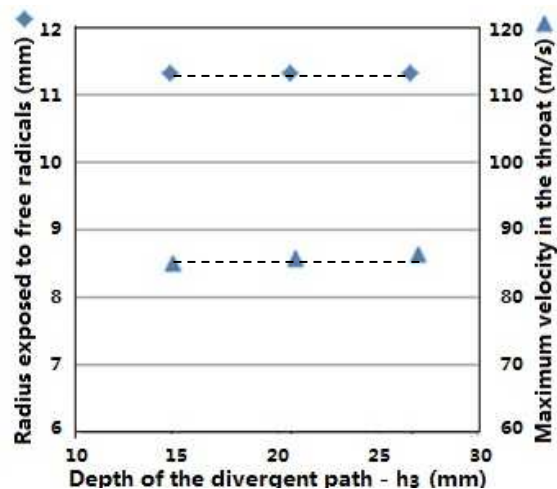
FIGURE 9. The depth of the divergent path ( h_3 ) versus the radius exposed to free radicals (♦ left), and h_3 versus the maximum velocity in the throat (▲ right). (Divergent angle changes with h_3 )
