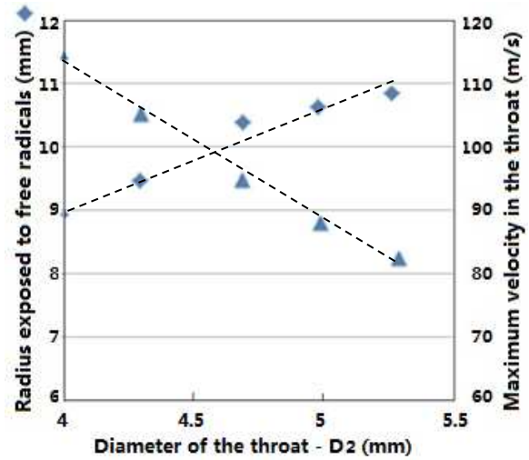
FIGURE 7. The throat diameter ( D_2 ) versus the radius exposed to free radicals ( \diamond left), and D_2 versus the maximum velocity in the throat ( \triangle right).
