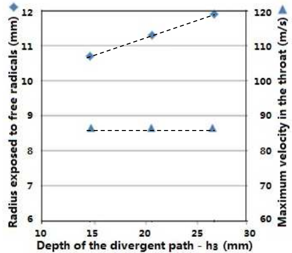
FIGURE 10. The depth of the divergent path ( h_3 ) versus the radius exposed to free radicals (♦ left), and h_3 versus the maximum velocity in the throat (▲ right). (Divergent angle is kept constant)
