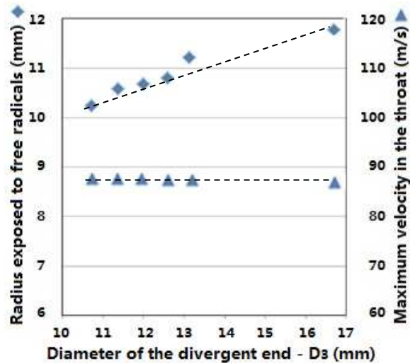
FIGURE 8. The divergent end dimensions ( D_3 ) versus the radius exposed to free radicals (♦ left), and D_3 versus the maximum velocity in the throat (▲ right).
