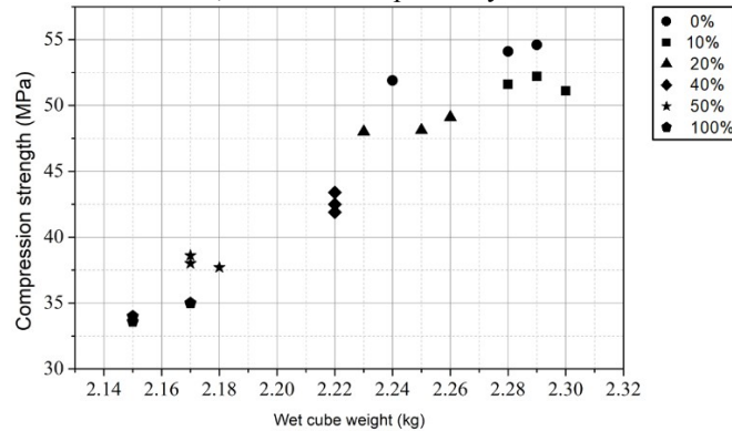
Fig. 2. Compression strength Vs wet cube weight (kg) for Wet cast
