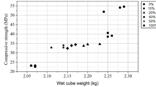
Fig. 4. Compression strength Vs wet cube weight (kg) for fibre-reinforced
