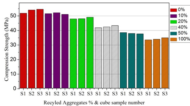
Fig. 1. Bar chart between Wet cast compression strength and % recycled aggregate replacement per sample
