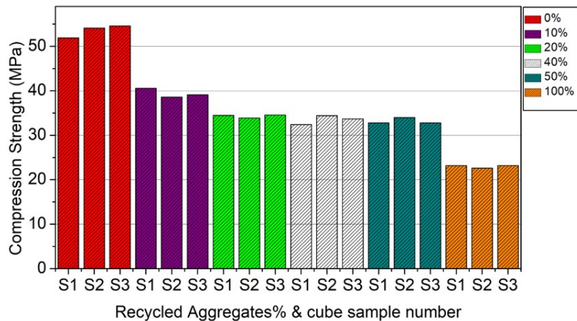
Fig. 3. Fibre compression strength Vs % recycled aggregate replacement per sample
