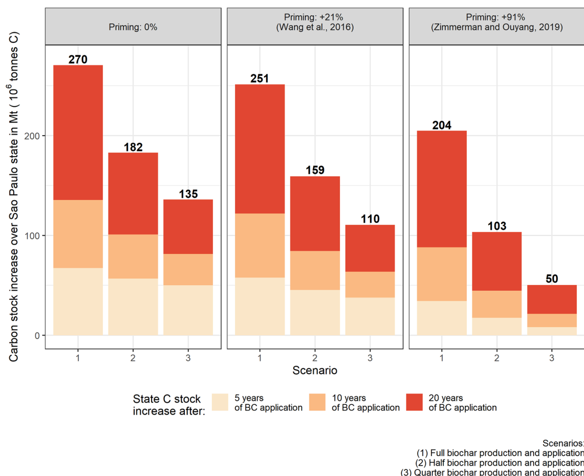
Figure 5. São Paulo State C sequestration potential. The number in bold above each bar represent the State total C sequestered after 20 year of biochar addition in Mt of C ( 10^6 t C).
