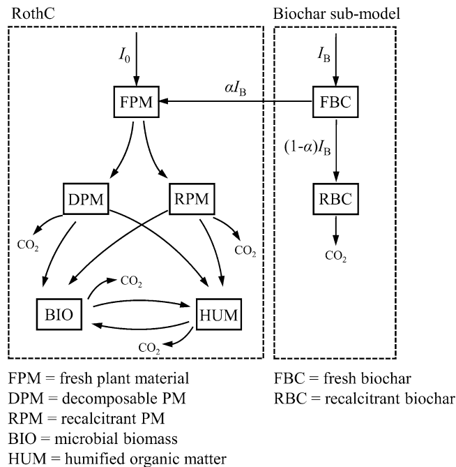
Figure 6. Soil carbon model. RothC is combined with a sub-model for the decomposition of fresh biochar. Details in text.
