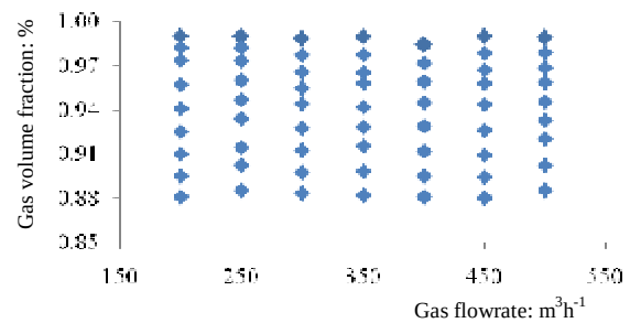
Fig 1 Wet gas test matrix
