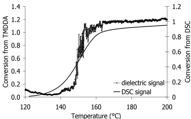
Fig. 6: Reaction conversion calculated from the TMDDA experiment ( A_T=1.5^\circ\text{C} , P=1.5\text{ min} , r=0.4^\circ\text{C/min} ). The reaction conversion obtained from DSC is also plotted for comparison.
