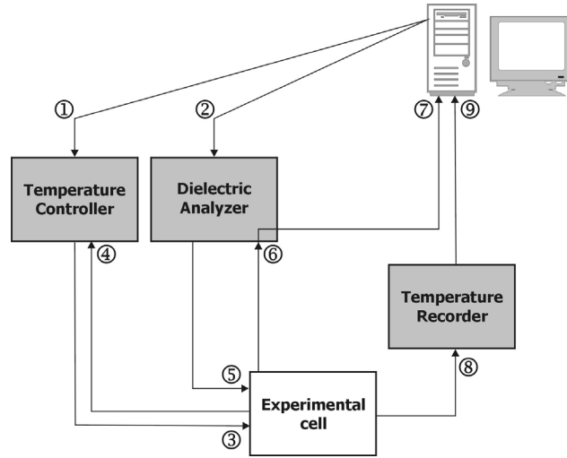
Fig. 2: Experimental setup for TMDDA measurements
