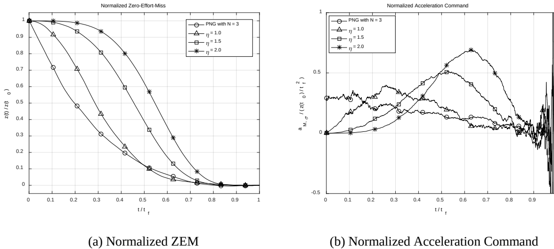
Fig. 6 Simulation results for a delayed correction pattern of ZEM in presence of seeker noise and autopilot lag
