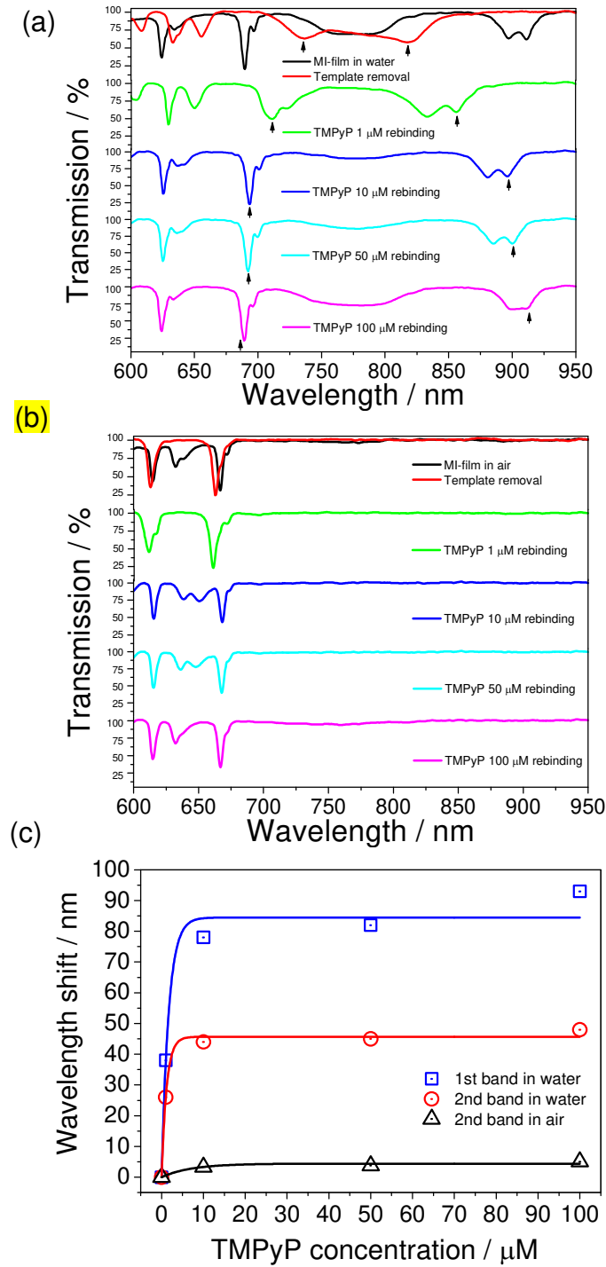
Figure 4. Transmission spectra of the MI-film-modified LPG upon rebinding with different concentrations of TMPyP in (a) water and (b) air. (c) Calibration curves plotted the from wavelength shifts of the 1st and 2nd resonance bands in water, and the 2nd resonance band in air. The arrows indicate the positions of the resonance bands.
