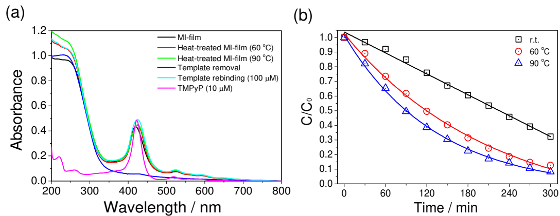
Figure 8. (a) UV–vis absorption spectra of the MI-film before and after heat treatment at 60 and 90 °C and upon TMPyP removal and rebinding in a 100 \mu M solution. The pink line shows the UV–vis spectrum of a TMPyP solution (10 \mu M). (b) The photodegradation of TMPyP on the MI-films, which are prepared without heat treatment (black line), with heat treatment at 60 °C (red line), and with heat treatment at 90 °C (blue line), under UV irradiation assessed from the absorbance at 422 nm.
