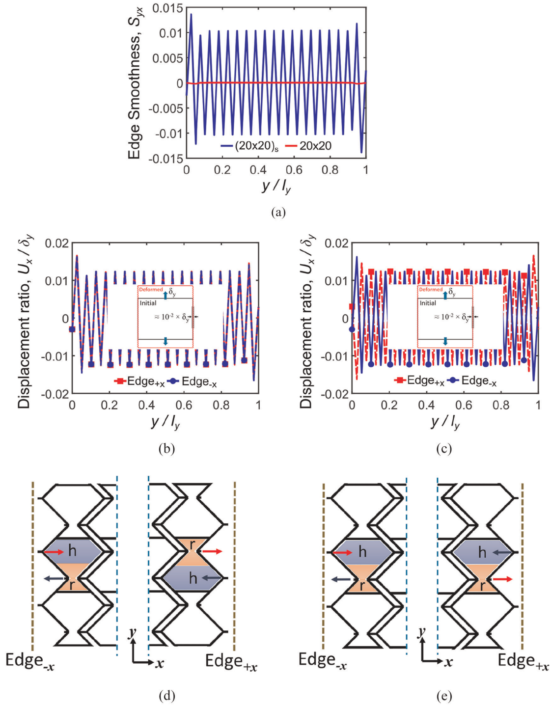
Figure 11. Edge smoothness S_{yx} analysis for loading in the y -direction: (a) for 20 \times 20 and (20 \times 20)_s tessellation numbers, (b) displacement ratio of nodes located on Edge _{+x} and Edge _{-x} for 20 \times 20 tessellation number, (c) displacement ratio of nodes located on Edge _{+x} and Edge _{-x} for (20 \times 20)_s tessellation number, (d) antisymmetric positions of re-entrant (r) and hexagonal (h) parts of the cell for asymmetric 20 \times 20 tessellation and the corresponding nodes' displacement vector, and (e) symmetric positions of re-entrant (r) and hexagonal (h) parts of the cell for symmetric tessellations and the corresponding nodes' displacement vector.
