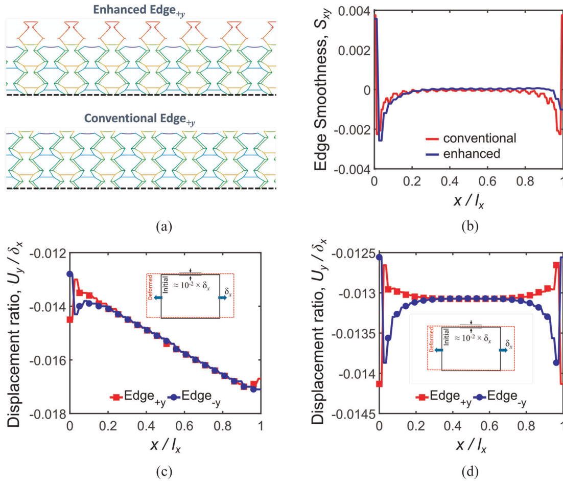
Figure 13. Edge enhancement effect on displacement ratio and edge smoothness S_{xy} : (a) enhanced and conventional edge deformations under tension in the x-direction, (b) comparison of edge smoothness S_{xy} for 20 \times 20 and (20 \times 20)^{\text{enhanced}} tessellations, (c) displacement ratio of corresponding nodes located on Edges \pm y for (20 \times 20)^{\text{enhanced}} tessellation, and (d) displacement ratio of corresponding nodes located on Edges \pm y for (20 \times 20)^{\text{enhanced}} tessellation.
