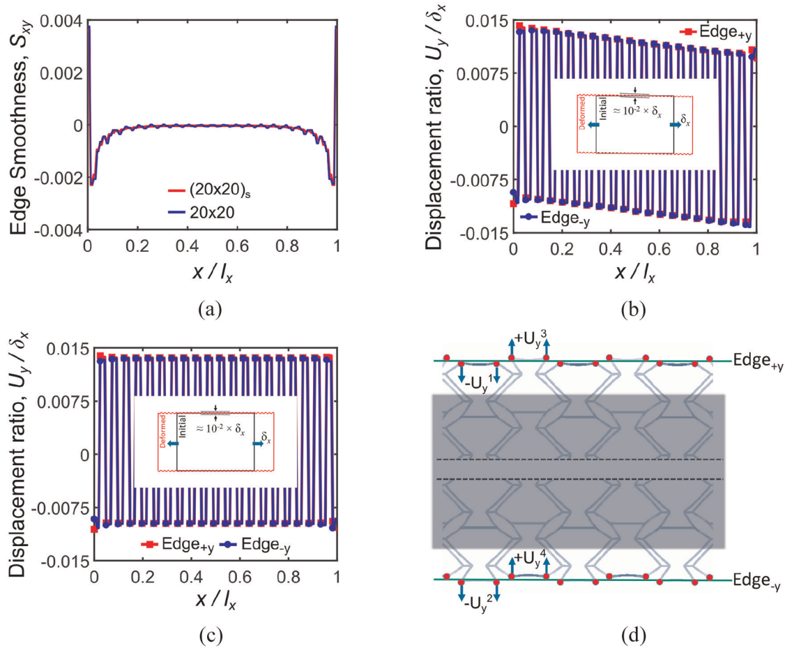
Figure 10. Edge smoothness S_{xy} analysis for loading in the x-direction: (a) for 20 \times 20 and (20 \times 20)_s tessellation numbers, (b) displacement ratio of nodes located on Edge +y and Edge -y for 20 \times 20 tessellation, (c) displacement ratio of nodes located on Edge +y and Edge -y for (20 \times 20)_s tessellation, and (d) schematic of displacements of the corresponding nodes on Edge +y and Edge -y .
