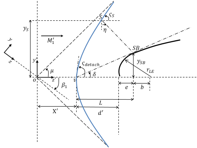
Figure 2 Hyperbolic approximation for a bow wave ahead of a blade-profile leading edge.
