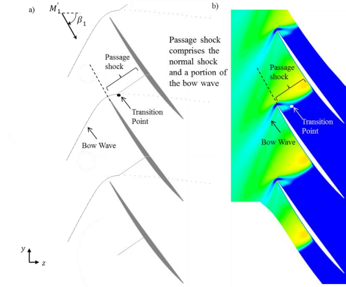
Figure 5 Transition point between the bow wave and the normal shock to form the passage shock. a) 2-D SLC simulation. b) 3-D CFD simulation.
