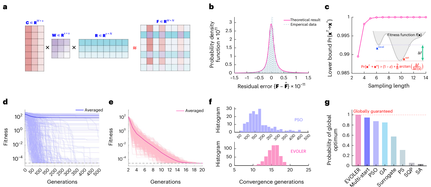
Fig. 2 | EVOLER enables globally guaranteed evolutionary computation.
