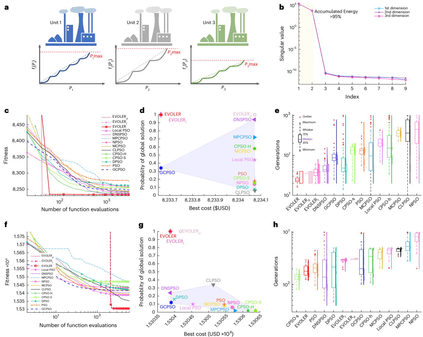
Fig. 5 | Optimal dispatch of power grid. a , Illustration of power dispatch with d=3 . b , Singular values of d -dimensional fitness ( d=3 ). c , Averaged results of various evolutionary computation methods ( d=3 , K=20 , 50 independent trials). d , Achievable minimal costs of different methods and the probabilities of finding them. e , Required generations for convergence (sample size 50).
