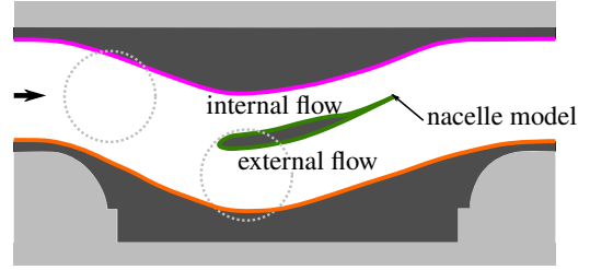
Fig. 3 Schematic generation of the rig geometry for both windmilling scenarios, with tunnel wall contours defined by streamlines extracted from a planar slice of 3D computations.
