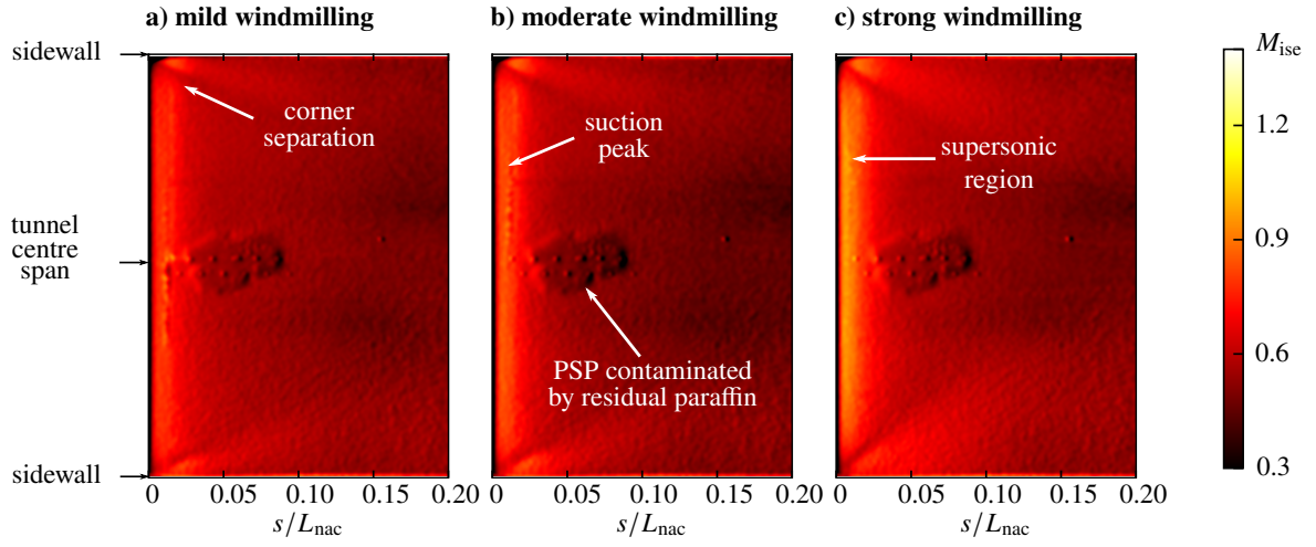
Fig. 17 Mach number distribution on the external surface for end-of-runway windmilling at Mach 0.25.
