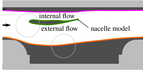
Fig. 3 Schematic generation of the rig geometry for both windmilling scenarios, with tunnel wall contours defined by streamlines extracted from a planar slice of 3D computations.
