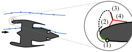
d) diversion windmilling (4.5° incidence, Mach 0.65) [5]
