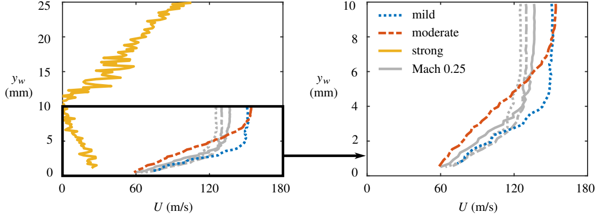
Fig. 24 Boundary-layer profiles from LDV at s = 0.24L_{nac} for end-of-runway windmilling at Mach 0.30.
