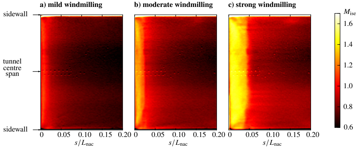
Fig. 11 Mach number distribution from PSP on the external surface for diversion windmilling at Mach 0.60.
