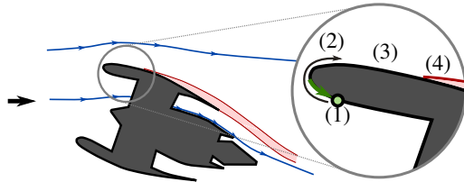
c) end-of-runway windmilling (20° incidence, Mach 0.25) [4]
