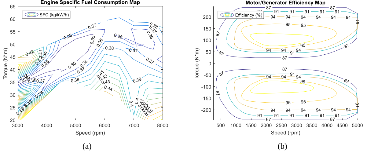
Fig. 4. Maps representing (a) specific fuel consumption, and (b) motor/generator efficiency
