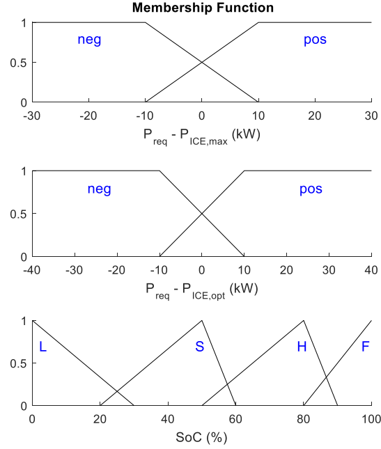
Fig. 5. Membership Functions
