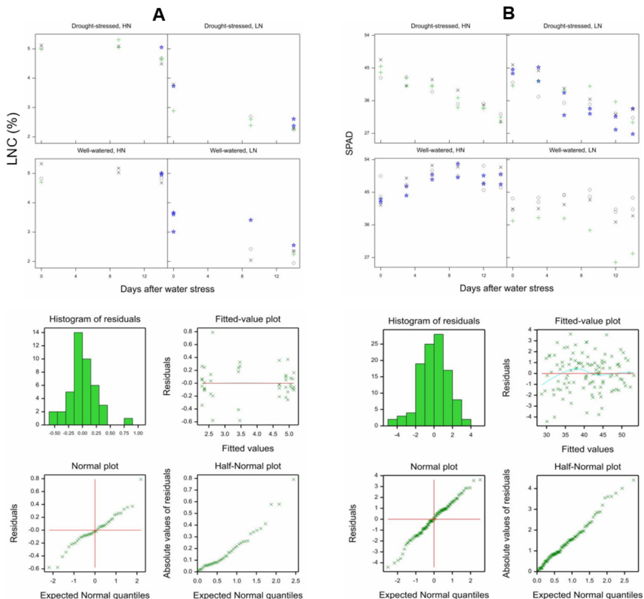
Figure C-1. Raw data distribution of the different treatments and residual plots of N stress morpho-physiological indicators in spring wheat. Raw data distribution and residual plots for (A) LNC and (B) SPAD. The residuals were inspected to verify the assumptions of normality (using histogram plots) and homogeneity of variance (using plots of fitted values).
