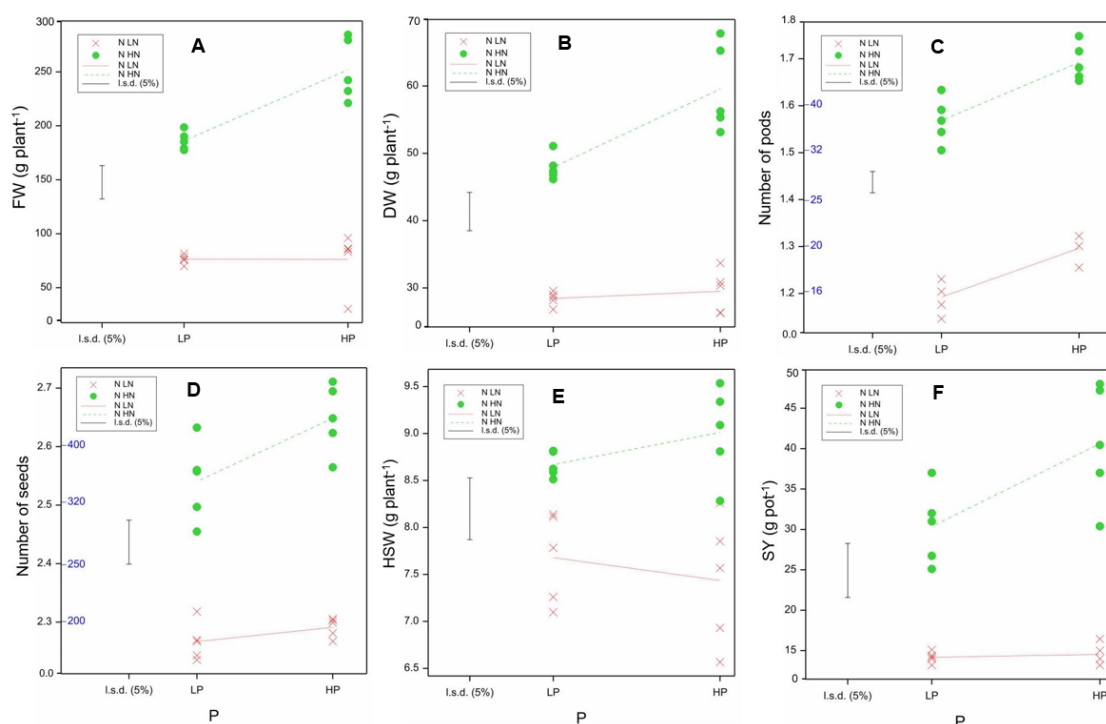
Figure 3.14. Responses of cowpea agronomic parameters including (A) FW, (B) DW, (C) number of pods, (D) number of seeds, (E) HSW and (F) SY. The mean and plotted values of the number of pods and number of seeds were transformed based on the log 10 scale to achieve homogeneity of the residuals. Mean values represent five replicates per treatment condition. Bars indicate the average least significant difference (LSD) at a 5% significance level.
