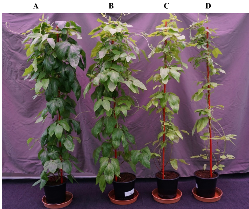
Figure 3.12. Morpho-physiological responses of cowpea assessed under different N and P availabilities. A, B, C and D indicate cowpea plants grown under HNHP, HNLP, LNHP and LNLP nutrient conditions respectively. The photograph was taken 74 days after sowing (DAS).
