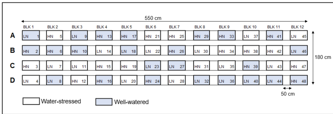
Figure 4.1. The statistical design used for the trial showing the allocation of the 2 \times 2 (i.e., N \times irrigation) factorial set of treatments according to a randomised complete block (BLK) design. The experimental area had dimensions of 550 \times 180 cm with 50 cm inter- and intra-row distance between pots. The rectangles are individual pots and those coloured in light blue were kept under well-watered (WW) conditions while non-coloured pots were water-stressed (WS). Pots are numbered from 1 to 48. LN = low N, HN = high N. A-D are individual rows.
