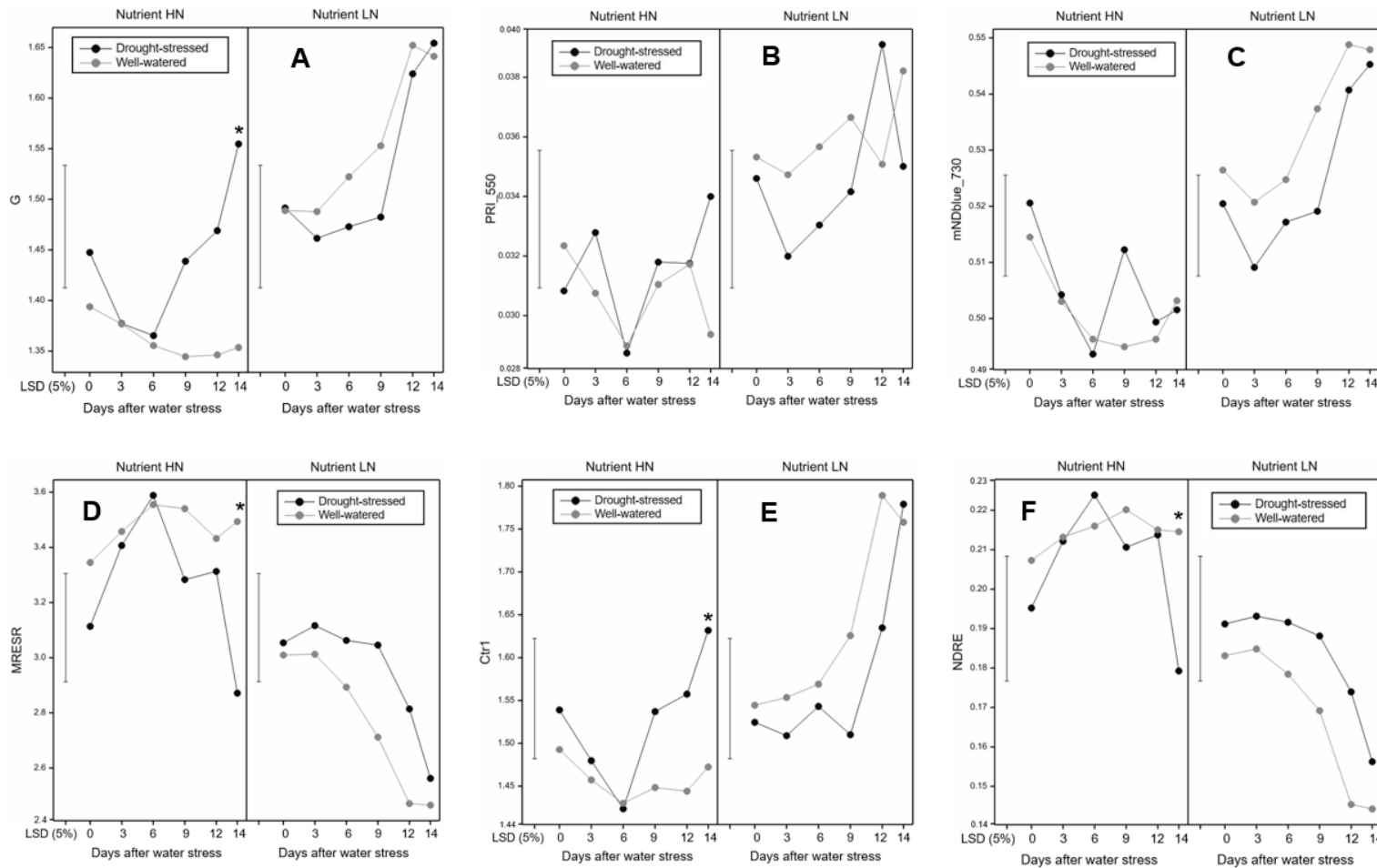
Figure 4.6. Time course of N responsive SRIs including (A) G, (B) PRI_550 (C) mNDblue_730, (D) MRESR, (E) Ctr1, (F) NDRE, and their drought responses under HN and LN nutrient conditions. Plotted means are estimations from the Autocorrelation (AR1) model. Bars represent average approximate LSDs with default significance set at a 5% level of REML means in each treatment combination and days after water stress (DAWS). Asterisks (*) indicate significant difference between drought-stressed and well-watered treatments under different N availabilities at 5% significance level.
