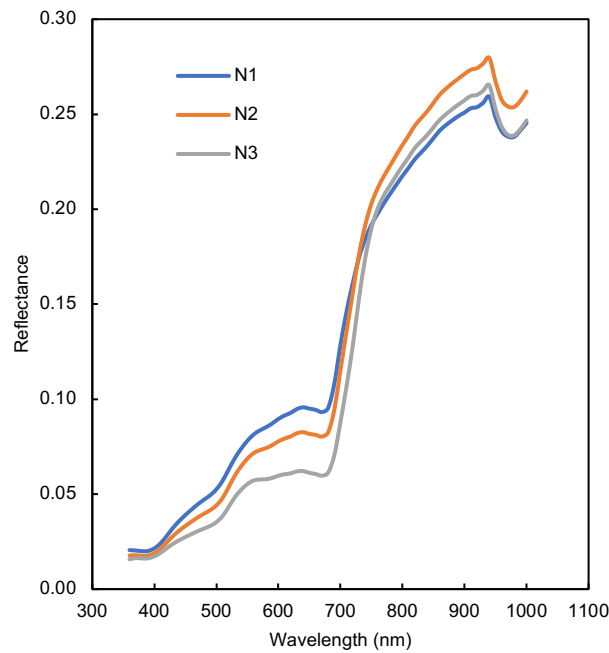
Figure 5.10. Reflectance spectra of winter wheat leaves exposed to different N levels and measured with the TEC5 spectrometer at anthesis. N1, N2 and N3 represent 100, 200 and 350 kg N ha -1 respectively.
