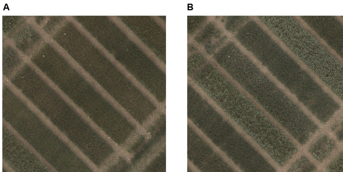
Figure 5.8. UAV imagery (orthomosaic) collected at a flying height of 25 m of (A) N1 (100 kg N ha -1 ) fertiliser treatment plots compared to (B) N3 (350 kg N ha -1 ) fertiliser treatment plots. Wheat cultivar Zyatt compared in both scenarios.
