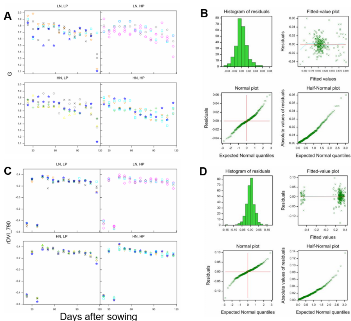
Figure B-7. Raw data distribution and residual plots of N stress-specific SRIs identified for cowpea. Raw data distribution for (A) G , residual plots for (B) G , raw data distribution for (C) rDVI_{790} and residual plots for (D) rDVI_{790} . The residuals were inspected to verify the assumptions of normality (using histogram plots) and homogeneity of variance (using plots of fitted values).
