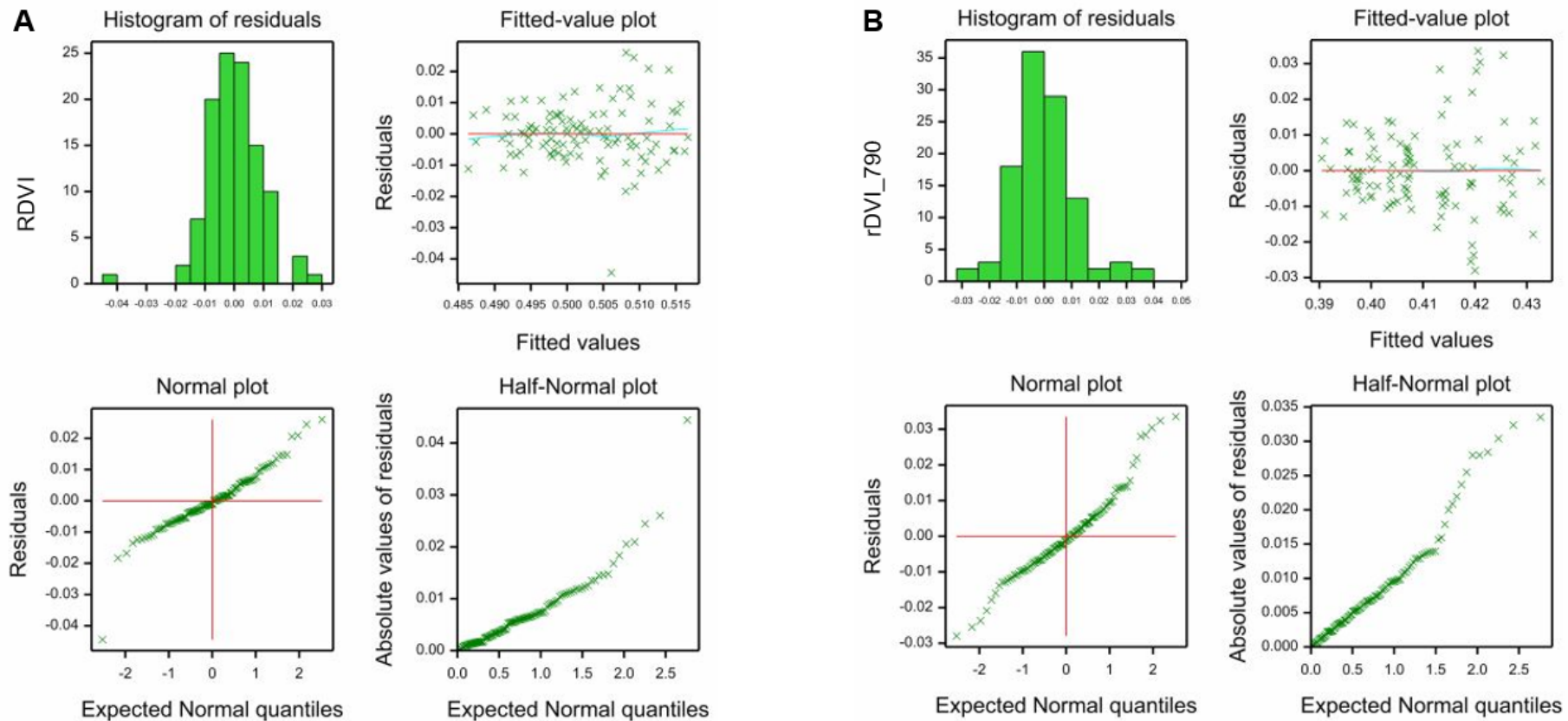
Figure C-6. Residual plots of drought stress-specific SRIs identified for spring wheat including (A) RDVI and (B) rDVI_790. The residuals were inspected to verify the assumptions of normality (using histogram plots) and homogeneity of variance (using plots of fitted values).
