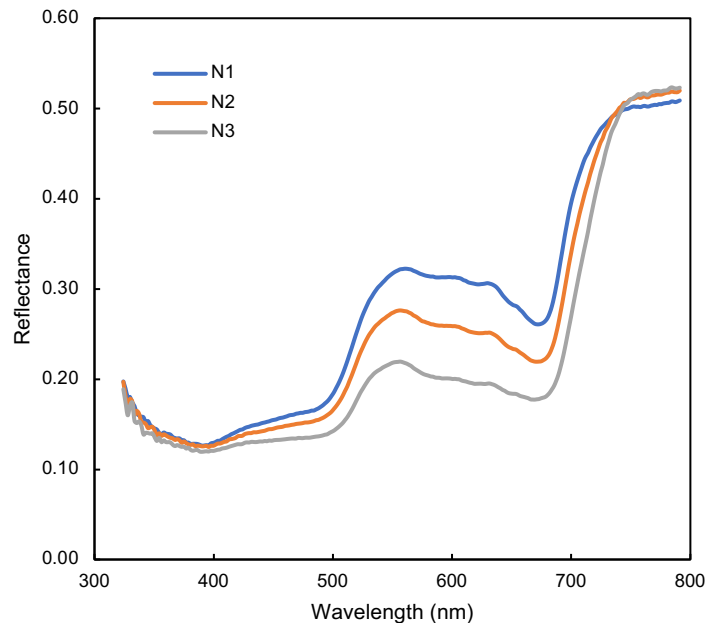
Figure 5.11. Reflectance spectra of winter wheat leaves exposed to different N levels and measured with the PolyPen RP410 spectrometer at anthesis. N1, N2 and N3 represent 100, 200 and 350 kg N ha -1 respectively.
