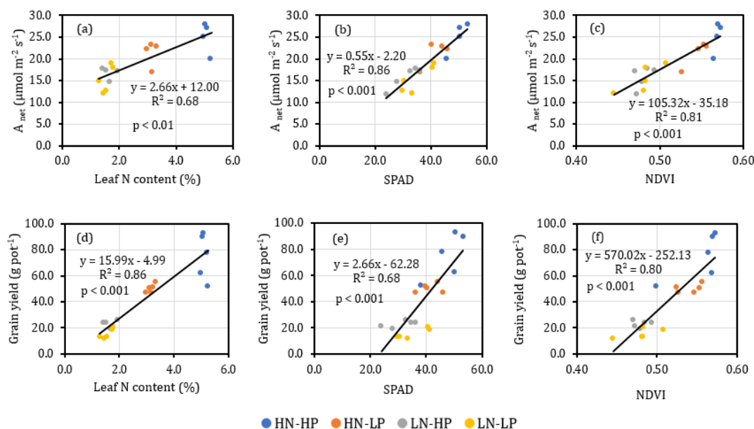
Figure 3. Correlations between leaf N content at 60 DAS and A_{\text{net}} at 46 DAS (a), SPAD at 46 DAS and A_{\text{net}} at 46 DAS (b), NDVI at 44 DAS and A_{\text{net}} at 46 DAS (c), leaf N content at 60 DAS and grain yield at harvest (d), SPAD at 46 DAS and grain yield at harvest (e), and NDVI at 44 DAS and grain yield at harvest (f). Each treatment represents five replicates, except HN-HP and HN-LP for A_{\text{net}} in which one of the replicates had wilted leaves and was removed. Significant levels are **p < 0.01 , ***p < 0.001 . SPAD and NDVI values are dimensionless.
