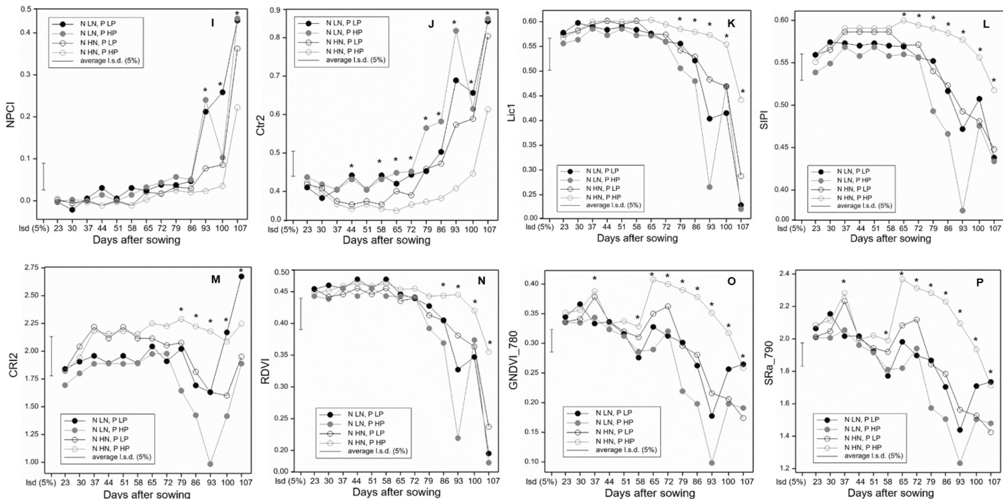
Figure 3.5. Time course of N stress responsive SRIs including (A) NDVI, (B) OSAVI, (C) G, (D) MCARI, (E) TCARI, (F) ZMI, (G) SPRI, (H) NPQI, (I) NPCL, (J) Ctr2, (K) Lic1, (L) SIPI, (M) CRI2, (N) RDVI, (O) GNDVI_780 and (P) SRa_790 showing their responses to N and P nutritional variations at specific days after sowing (DAS) during quinoa crop cycle from 23 to 107 DAS. Mean values represent five replicates per treatment condition. Bars indicate the average least significant difference (LSD) at the 5% significance level. Asterisks (*) indicate significant difference between treatments at 5% significance level at different DAS.
