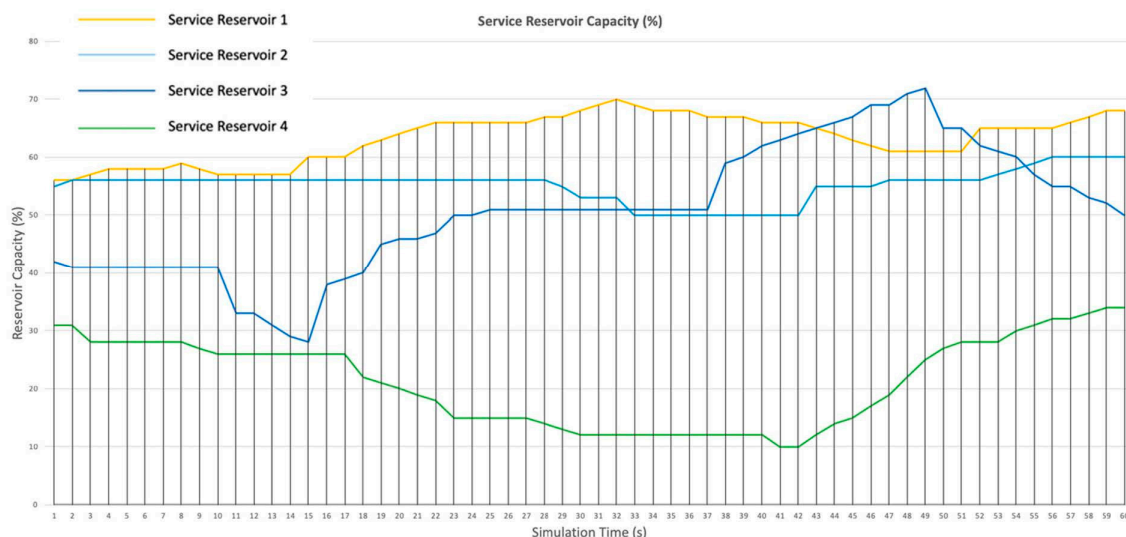
Figure 14. Service reservoir capacity from simulation run.
