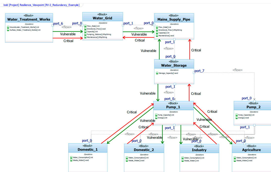
Figure 11. RV-2—Two pump architecture solution.
