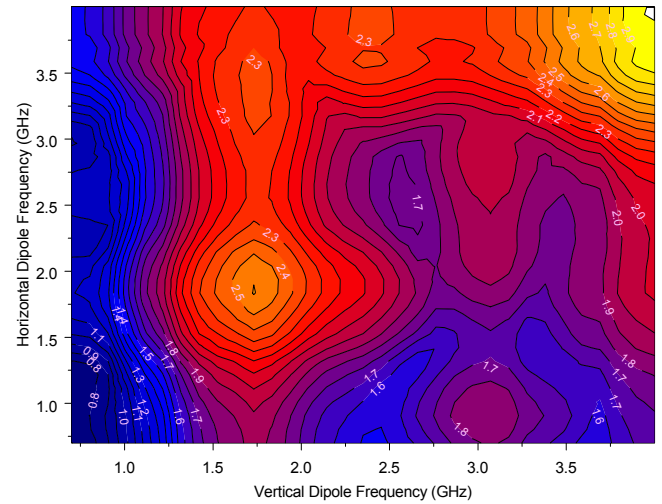
Figure 5. Combined 1g SAR with one horizontal dipole and one vertical dipole in front of the face.
