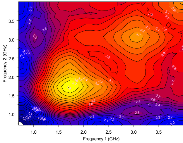
Figure 3. Combined 1g SAR with two vertical dipoles
