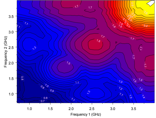
Figure 4. Combined 1g SAR with two horizontal dipoles
