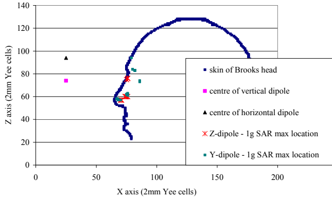
Figure 2. The location of the maximum 1g SAR in the head with Y and Z dipoles.
