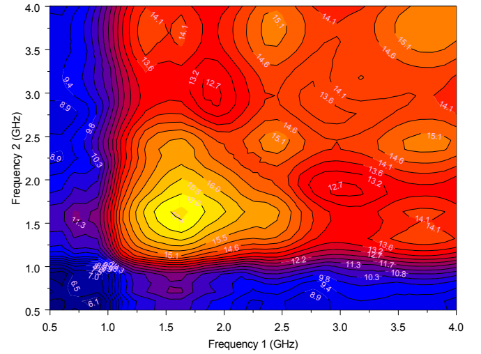
Figure 1. Combined 1g SAR from two vertically polarised plane wave sources.
