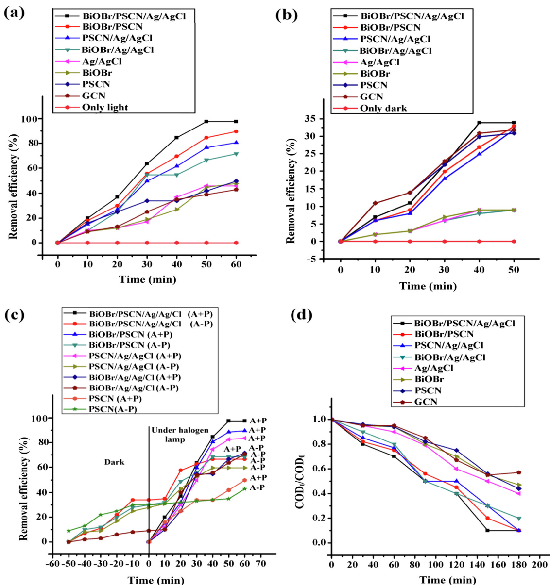
Fig. 7 (a) Photocatalytic degradation of phenol, (b) adsorptional removal of phenol, (c) time profile for removal of phenol under three reaction conditions and (d) COD removal. Reaction conditions: [phenol] = 1 \times 10^{-4} mol dm ^{-3} ; [photocatalyst] = 50 mg/100 mL; initial reaction pH = 4.0 and Light intensity = 750 lx.
