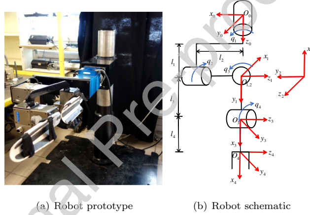
Figure 3: 4-DOF robot
