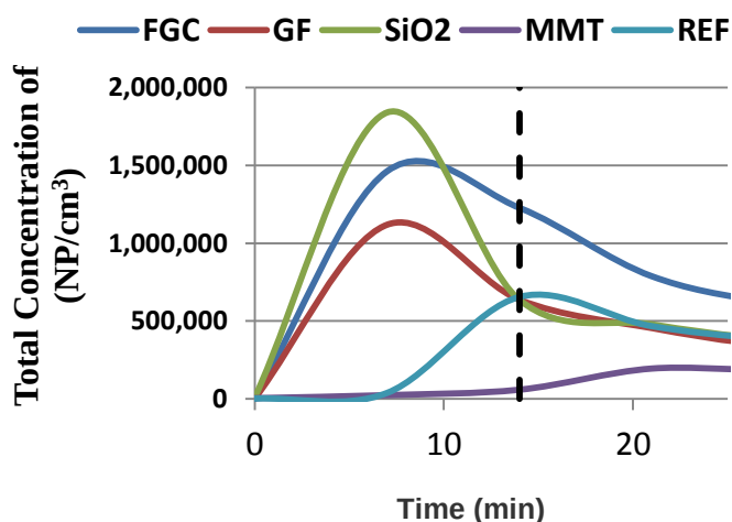
Figure1. Monitoring of air borne NP generated during drilling of PA6 group of specimens. The lines represent NP released from PA6 reinforced with silica NP (SiO 2 ), microfiller of montmorillonite (MMT), foam glass crystal (FGC), and glass fiber (GF). PA6 polymer was used as a reference (REF).
