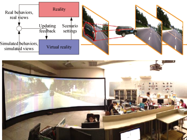
Fig. 7. Realization and demonstration of parallel testing.
