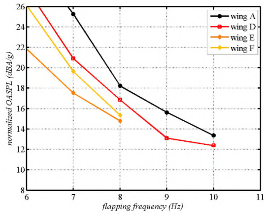
Figure 7: Performance of wings A, D, E, and F at various flapping frequencies: a) OASPL; b) thrust; c) OASPL per unit thrust. The noise was measured at 90°.
