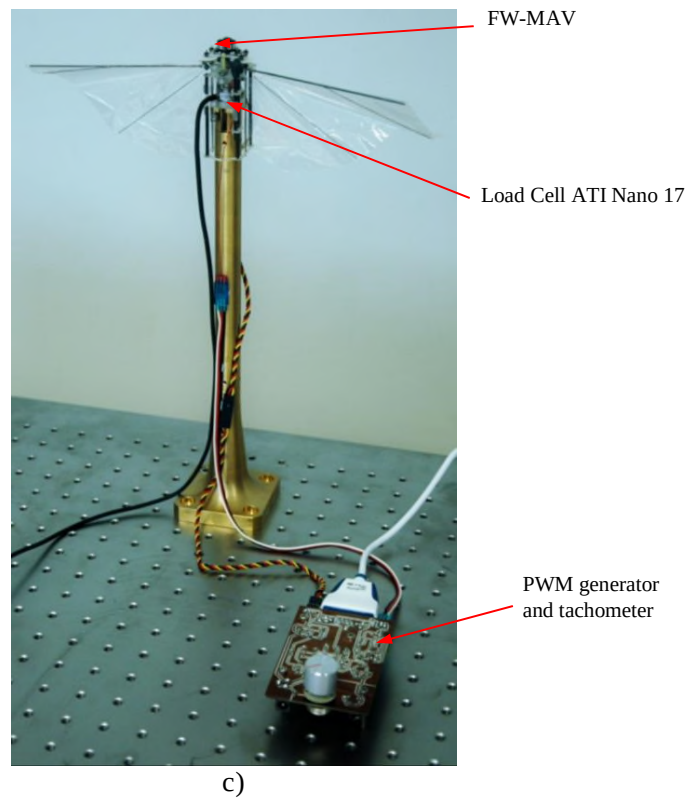
Figure 4: Experimental setup: a) side view and b) top view of the placement of the flapping-wing model and microphones inside the anechoic chamber; c) time-dependent thrust measurement system.
