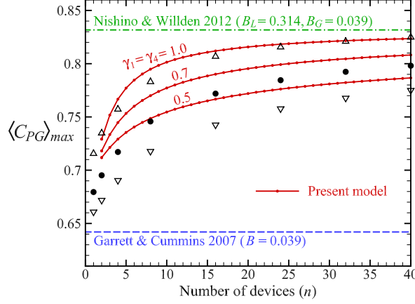
FIGURE 10. Effect of the number of devices on the maximal global power coefficient: obtained from RANS computations ( \triangle : C_{\epsilon 1} = 1.36 ; \bullet : C_{\epsilon 1} = 1.44 ; \nabla : C_{\epsilon 1} = 1.52 ) and analytical models; for s/d = 0.25 .
