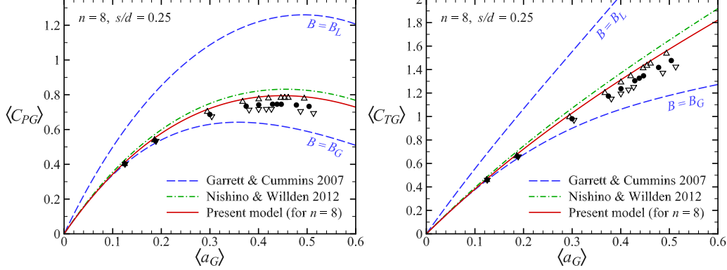
FIGURE 9. Comparisons of global power and thrust coefficients between RANS computations ( \triangle : C_{\epsilon 1} = 1.36 ; \bullet : C_{\epsilon 1} = 1.44 ; \nabla : C_{\epsilon 1} = 1.52 ) and analytical models; for n = 8, s/d = 0.25 .
