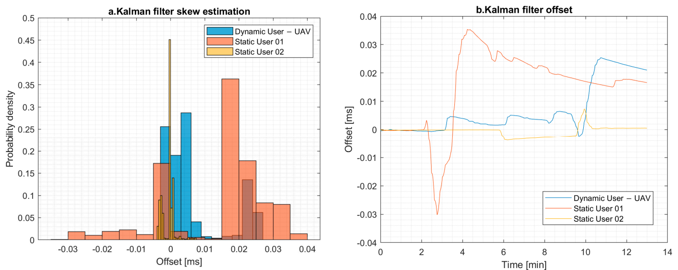
Figure 4. Kalman Filter offset estimation for two static users and one dynamic user.
