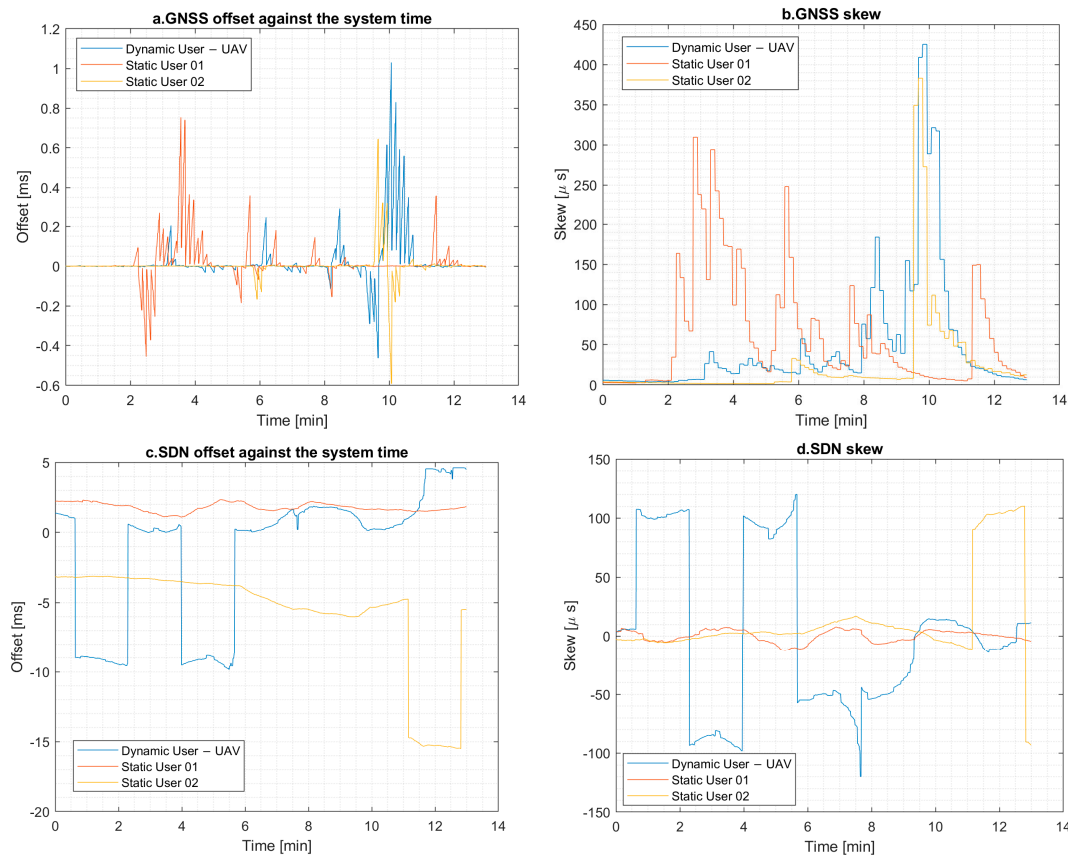
Figure 3. GNSS and SDN performance for two static and dynamic users within the same network.
