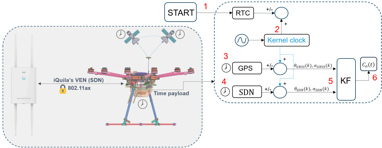
Figure 1. Time fusion framework using GNSS and iQuila's VEN time data as alternative time source. 1—Start the local embedded board; 2—Kernel clock adjusted with the RTC mechanism; 3—GPS time source; 4—SDN time source; 5—KF input data; 6—KF output.
