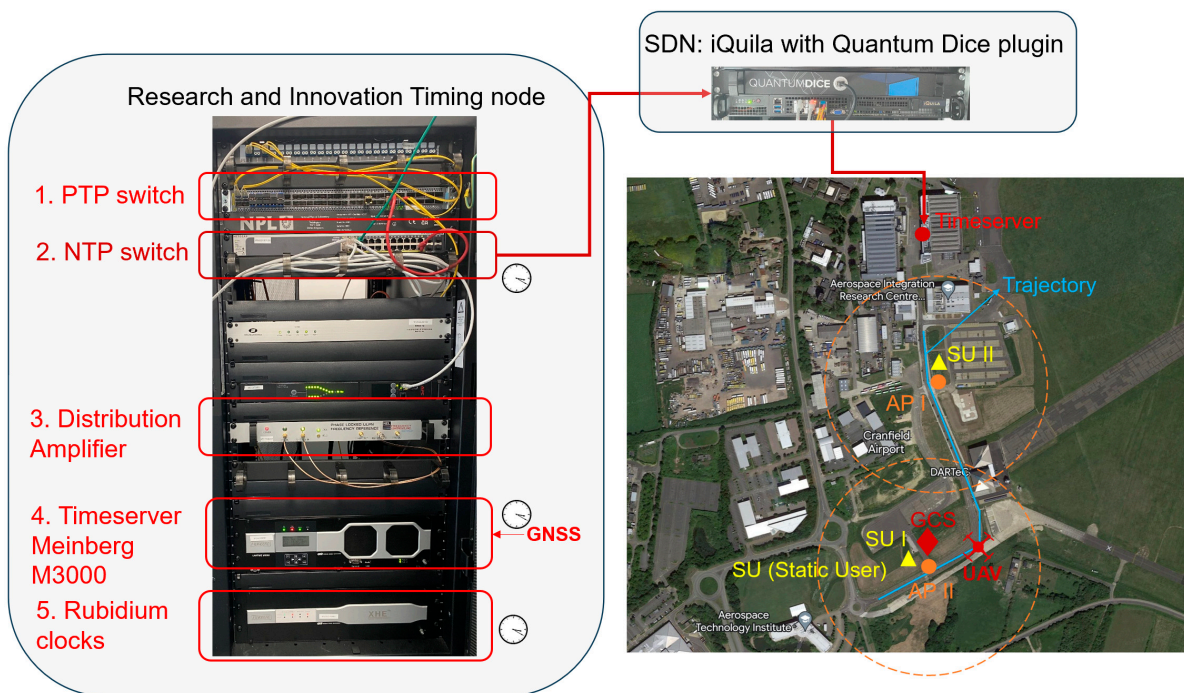
Figure 2. Practical system configuration in an outdoor environment.
