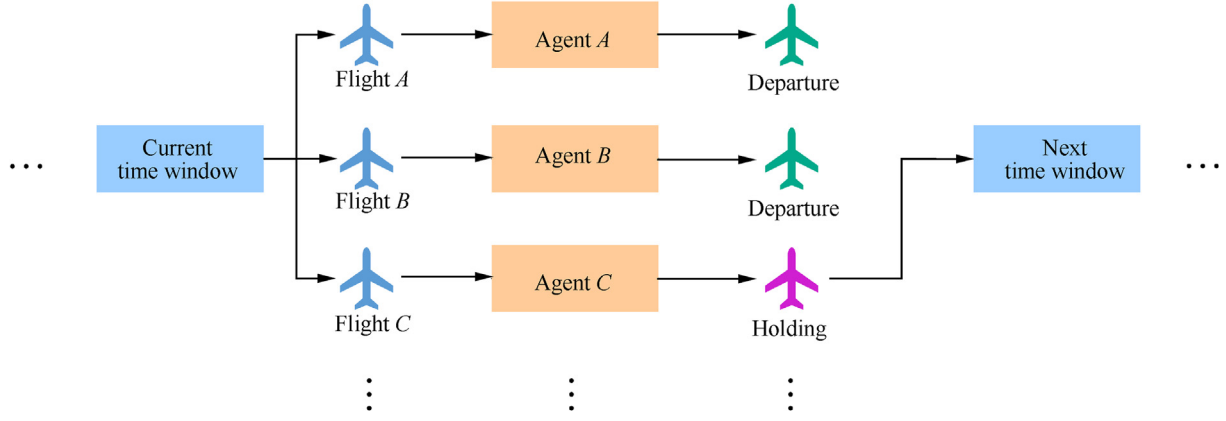
Fig. 3 Multi-agent decision-making framework (top-level framework of the proposed method) where all agents are distributed.
