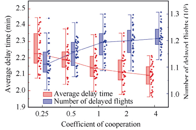
Fig. 13 Experimental results of sensitivity analysis on coefficient of cooperation.
