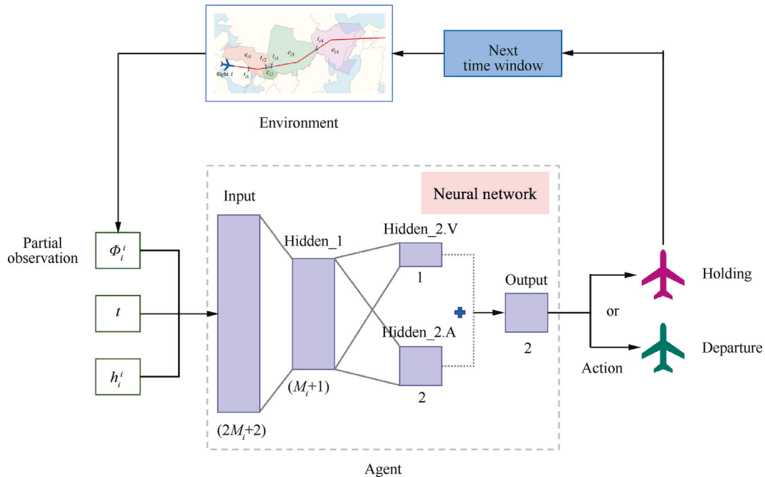
Fig. 4 Architecture of policy network, showing the working process of an agent and focusing on neural network.
