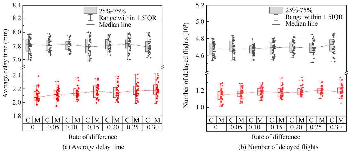
Fig. 10 Experimental results of method generalisation test for flight schedules.
