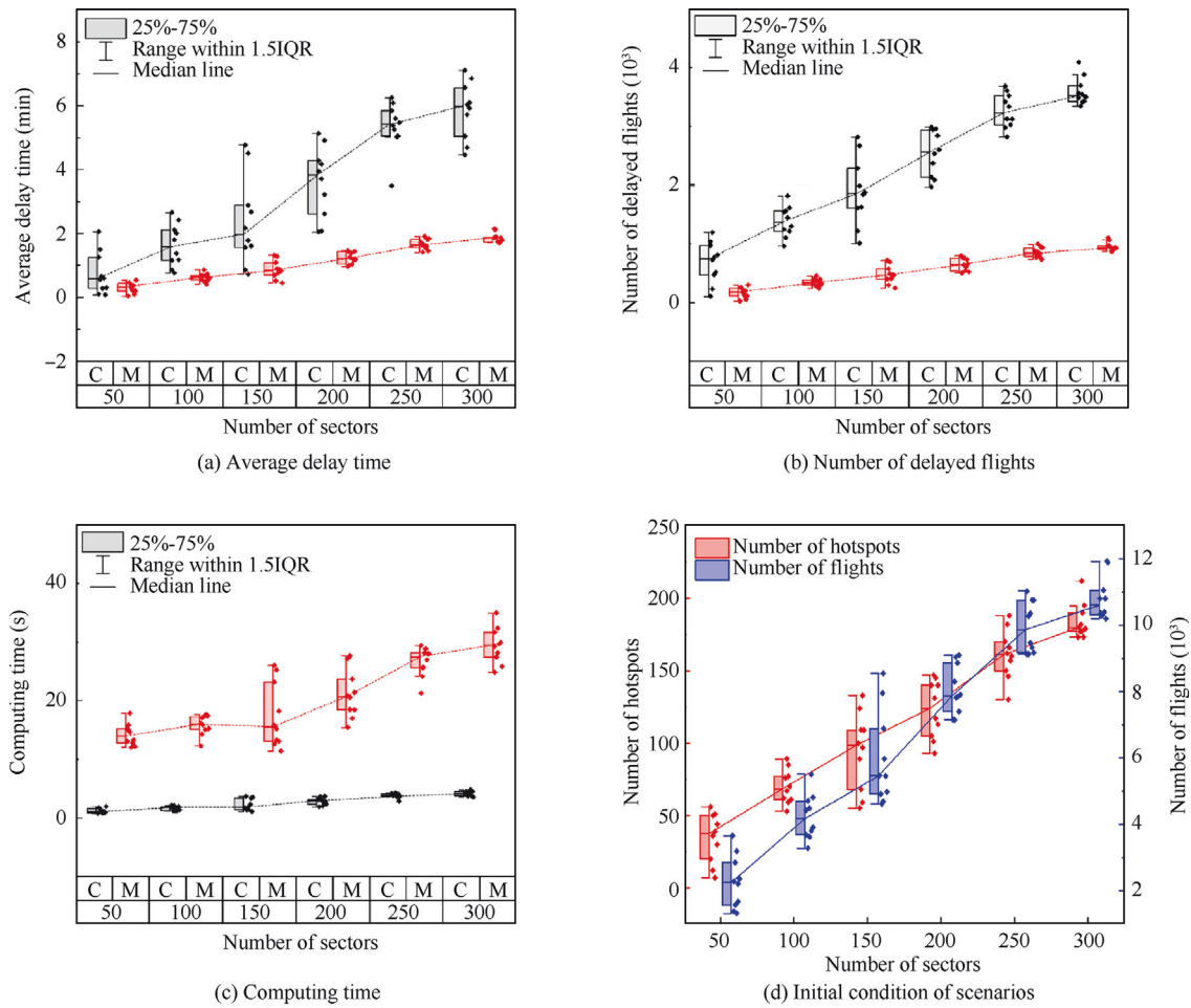
Fig. 11 Experimental results of method generalisation test for problem scales.
