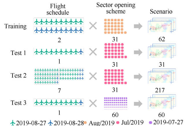
Fig. 8 Scenarios generation for performance tests.
