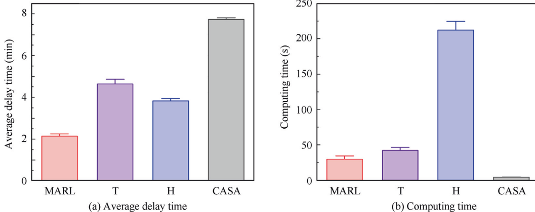
Fig. 12 Experimental results of the comparison of RL-based DCB methods.
