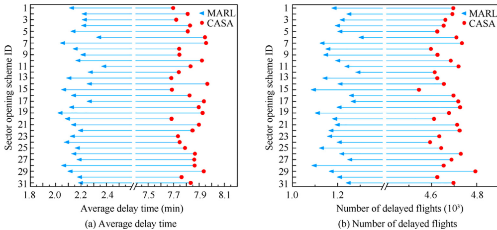
Fig. 9 Experimental results of method generalisation test for sector opening schemes.
