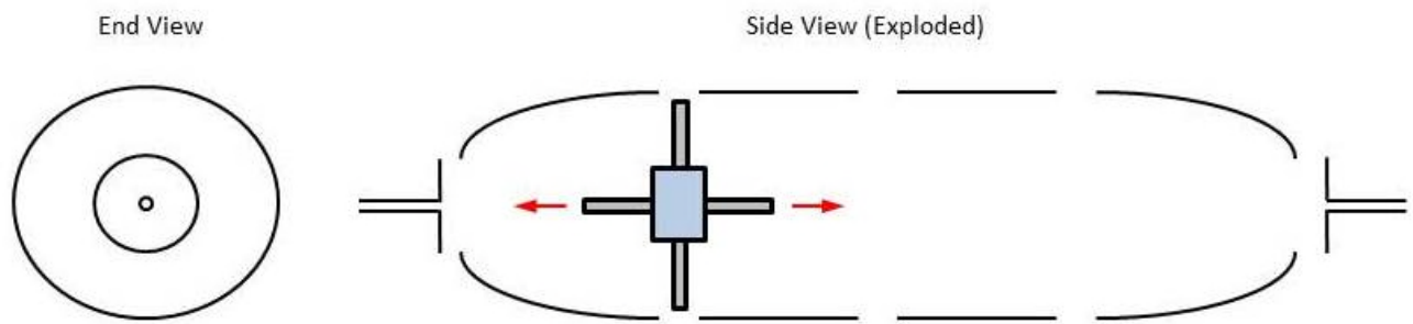
Figure 16 – Modified tank design. The exploded view shows a tank cross-section and the weld joint locations. An increased opening at each end would allow more access for internal fixtures.
