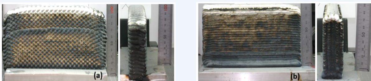
Figure 4: Physical quality of aluminium 2319 WAAM walls produced: (a) oscillated deposited wall; (b) parallel deposited wall
