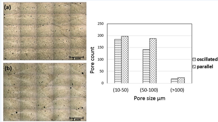
Figure 8: Pore distribution in as-deposited (a) oscillated and (b) parallel walls.
