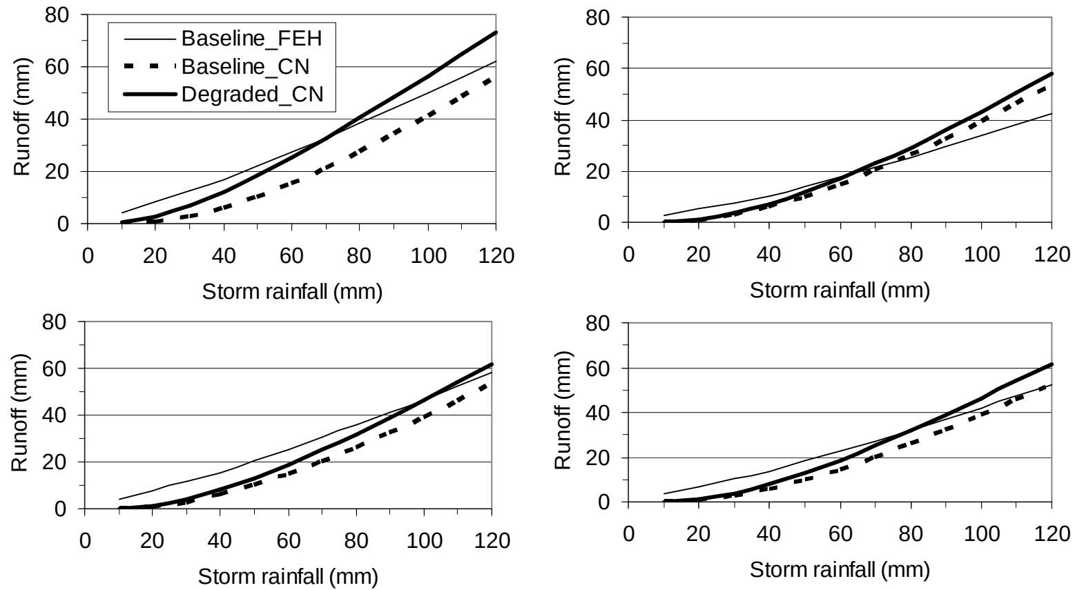
Figure 4 Potential increase in runoff caused by a soil structural degradation for a range of rainfall events calculated using a Curve Number approach for the (top left) Uck, (top right) Bourne, (bottom left) Yorkshire Ouse and (bottom right) Severn catchments
