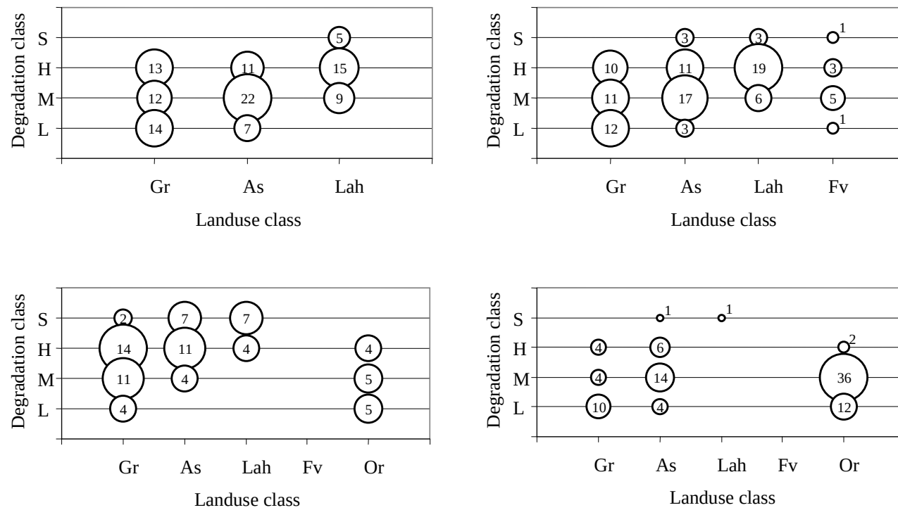
Figure 2 Distribution of observed Soil Degradation Class by management system in the (top left) Yorkshire Ouse, (top right) Severn, (bottom left) Uck and (bottom right) Bourne catchments
