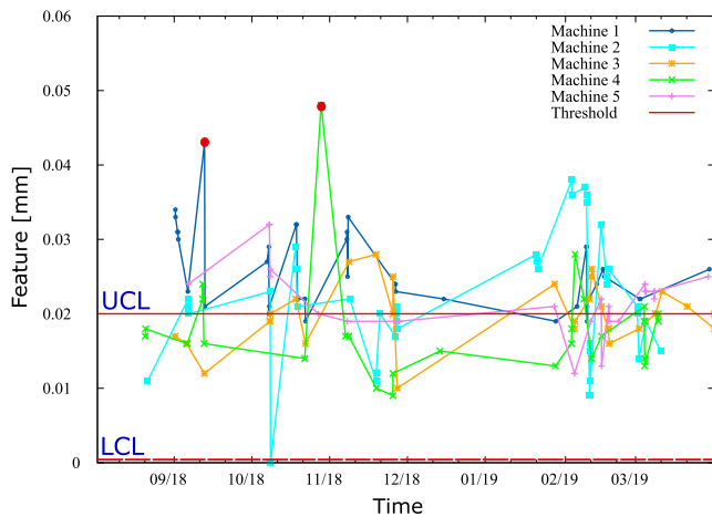
Fig. 2. Outliers (red dots) identified on CMM measurements of a particular feature F corresponding to 5 machines. Although the algorithm picks up an outlier in machine A_7_1, this measurement is not considered an outlier in this particular case as the target value for this feature is zero. (For interpretation of the references to colour in this figure legend, the reader is referred to the web version of this article.)
