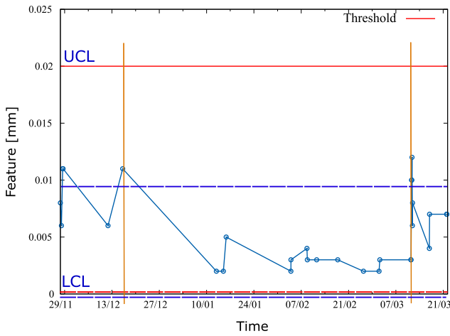
Fig. 4. Detected shifts on a subset of measurements of a sample feature and machine. Each vertical line indicates the point in time where the change is detected. Two moments are identified here, one where there is a tendency towards the target value, which is zero, and one where the measurements start to move away.
