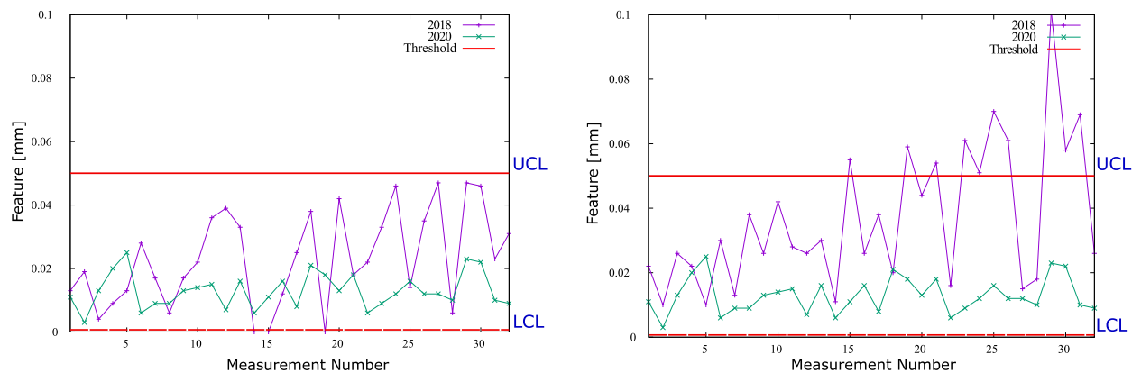
Fig. 10. Thirty two consecutive measurements of a single feature captured for Machine 1 (left) and Machine 2 (right) during the periods 2018 and 2020. As a unilateral tolerance, the target value in both cases is zero.
