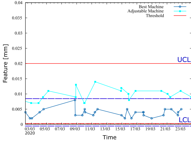
Fig. 3. Example where machine A_4_1 is identified as the best machine (closer to the target value zero) and A_3_2 is identified as one of the adjustable machines.
