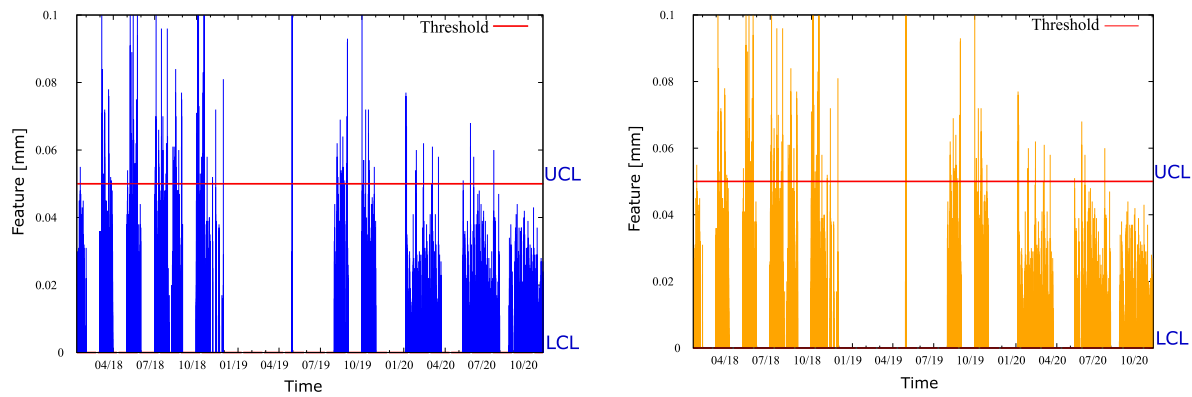
Fig. 9. Measurements of a single feature captured for Machine 1 (left) and Machine 2 (right) during the period 2018–2020. For both machines, the target value is zero and the upper limit tolerance is shown with a red horizontal line.
