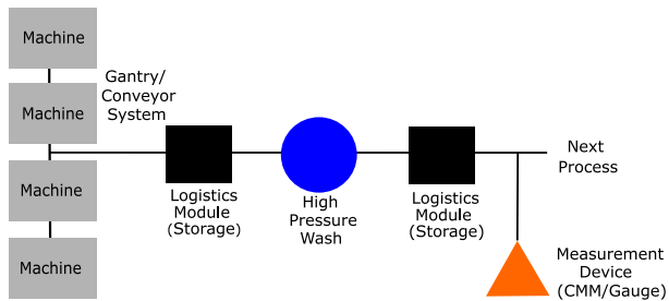
Fig. 7. Selected parts for measurement move through a conveyor system in order to be high-pressure washed before they go through the measurement process.
