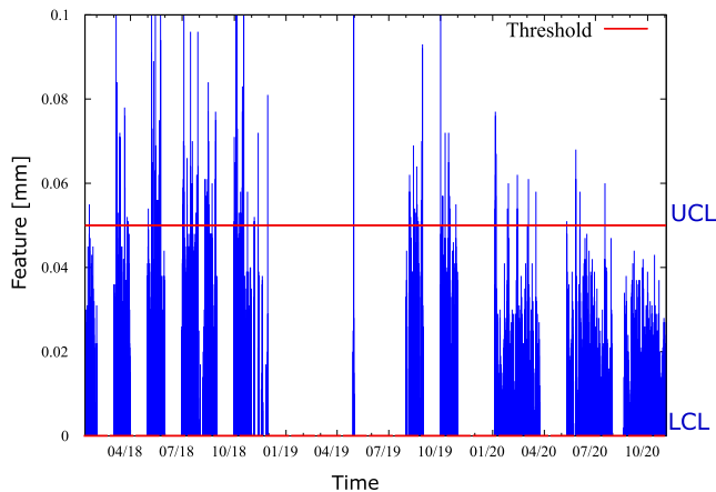
Fig. 8. Measurements of a single feature captured for all monitored machines during the period 2018–2020. For this feature, the upper limit tolerance is indicated with a horizontal red line, and the target value is zero. (For interpretation of the references to colour in this figure legend, the reader is referred to the web version of this article.)
