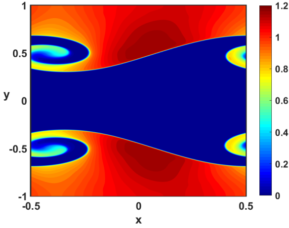
(c) 512 \times 1024 : MP-WENO7
