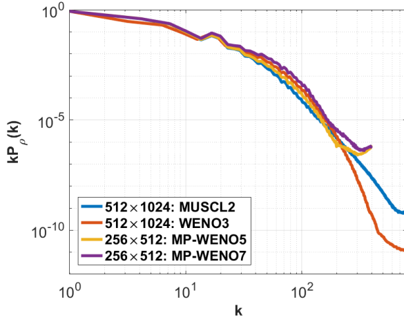
(a) Coarser grid comparative.
