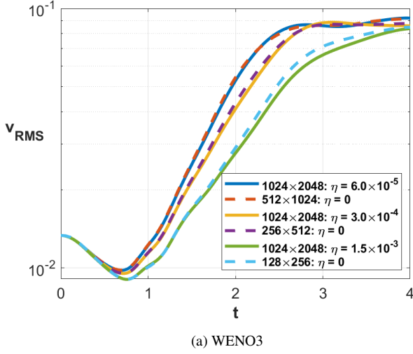
Figure 11. Evolution of the v_{\text{RMS}} for different grid resolutions and values of \eta for the WENO3 (11a) and MP-WENO5 (11b) schemes.
