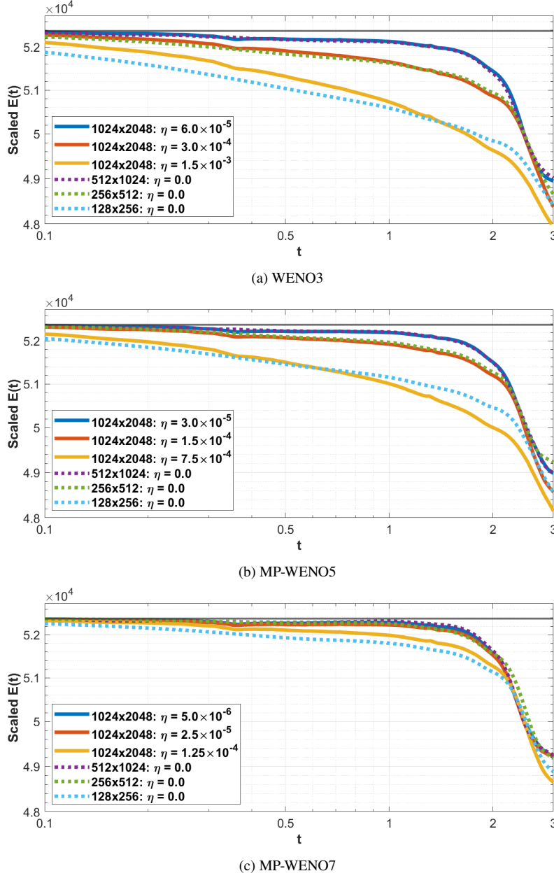
Figure 5. Time-evolution of the total kinetic energy in the system at different grid resolutions and different values of \eta for the WENO3 (5a), MP-WENO5 (5b), and MP-WENO7 (5c) schemes.
