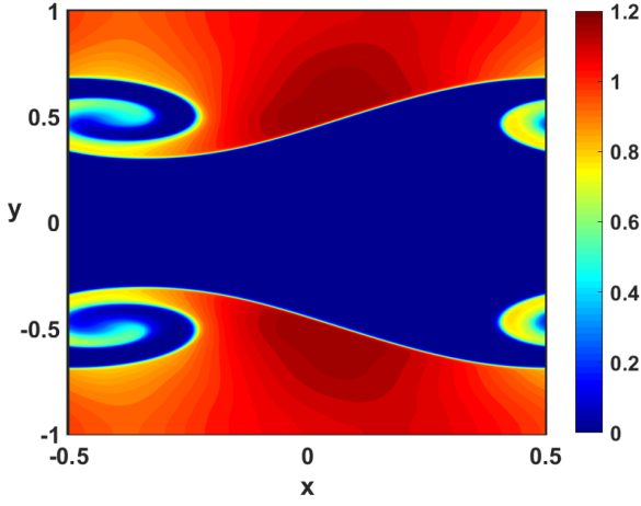
(a) 512 \times 1024 : MP-WENO5
