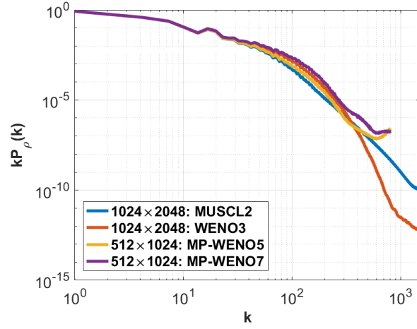
(b) Finer grid comparative.
