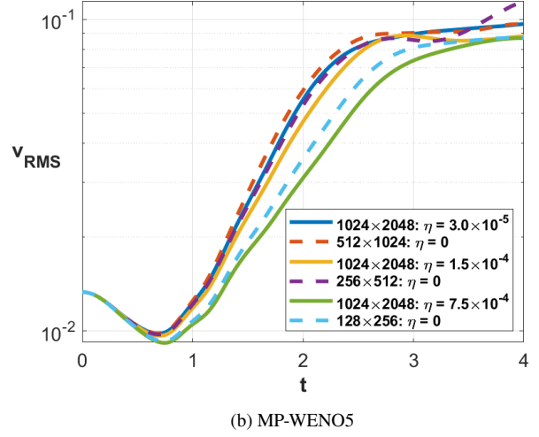
Figure 11. Evolution of the v_{\text{RMS}} for different grid resolutions and values of \eta for the WENO3 (11a) and MP-WENO5 (11b) schemes.
