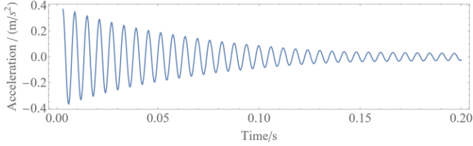
Figure 10: THE OUTPUT FROM THE FILTER CORRESPONDING TO THE INPUT OF FIGURE 9
