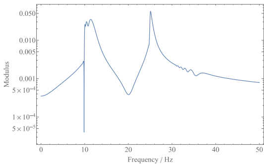
Figure 15: THE SPECTRUM OF THE TIME SERIES FOR A NONLINEAR SYSTEM
