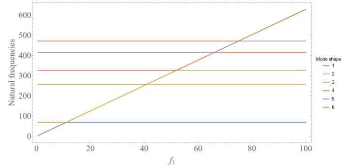
Figure 4: THE NATURAL FREQUENCIES OF A SYSTEM WITH SIX DEGREES-OF-FREEDOM WITH VARYING STIFFNESS MATRIX
