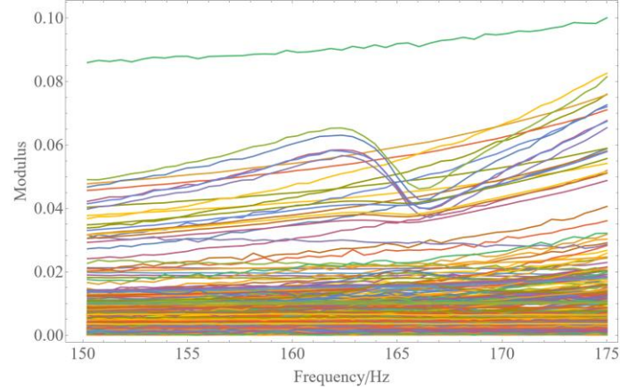
Figure 8: EXPANDED VERSION OF FIGURE 7 HIGHLIGHTING THE MODE AT APPROXIMATELY 165 HZ.
