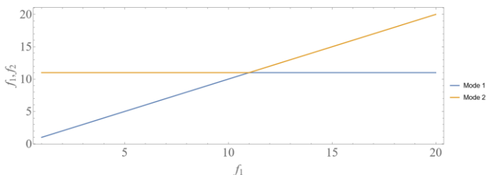
Figure 3: THE NATURAL FREQUENCIES WITH VARYING STIFFNESS MATRIX
