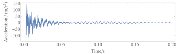
Figure 9: A TIME HISTORY FROM THE IMPULSE EXCITATION
