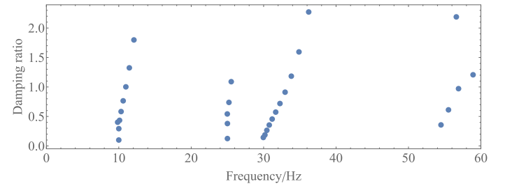
Figure 17: THE NATURAL FREQUENCIES AND DAMPING RATIOS OF THE MODEL FITTED TO THE SPECTRUM OF FIGURE 15.
