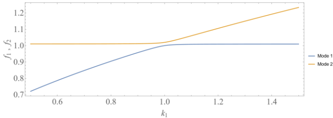
Figure 2: THE NATURAL FREQUENCIES AS A FUNCTION OF SPRING STIFFNESS.
