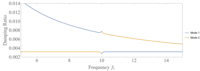
Figure 6: The DAMPING RATIO AS A FUNCTION OF NATURAL FREQUENCY OF A TWO DEGREE-OF-FREEDOM SYSTEM
