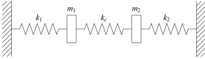
Figure 1: A TWO DEGREE OF FREEDOM SYSTEM WITH SPRINGS AND MASSES
