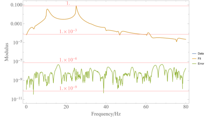
Figure 20: THE SPECTRUM, THE FIT AND THE ERROR.
