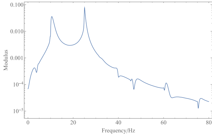
Figure 19: THE SPECTRUM OF A COUPLED NONLINEAR SYSTEM
