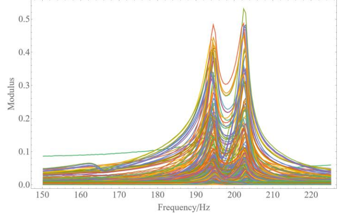
Figure 7: MEASURED SPECTRA FROM IMPULSE EXCITATION THERE ARE THREE MODES IN THE FIGURE
