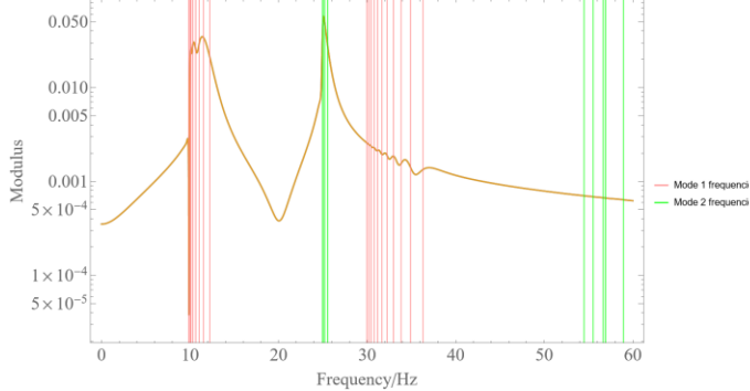
Figure 18: THE SPECTRUM WITH FITTED FREQUENCIES IDENTIFIED WITH MODES.
