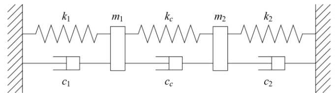
Figure 5: A TWO DEGREE OF FREEDOM SYSTEM WITH SPRINGS, DAMPERS AND MASSES. EXTERNAL FORCES MAY BE APPLIED TO THE MASSES TO GENERATE MOTION.
