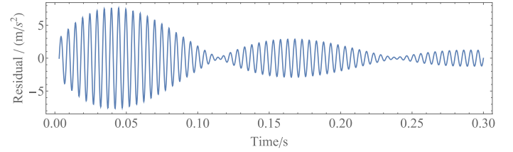
Figure 13: THE FILTERED DATA FROM THE TIME HISTORY OF FIGURE 9.
