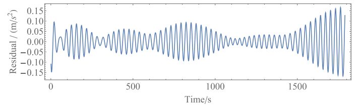
Figure 14: THE RESIDUAL FOLLOWING FITTING OF THE MODEL IN EQUATION 5 TO THE DATA IN FIGURE 13.
