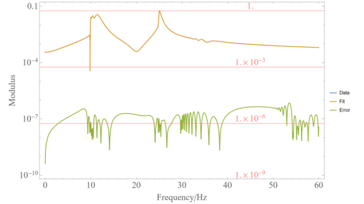
Figure 16: THE SPECTRUM, THE FITTED MODEL AND THE ERROR
